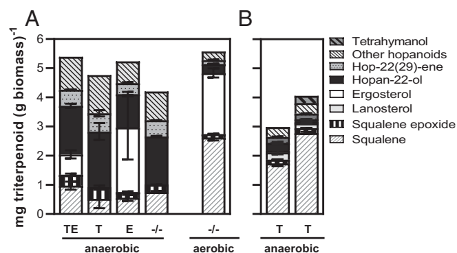
Fig. 4. Quantification of triterpenoids in yeast biomass. (A) Triterpenoid content of cultures of Sch. japonicus CBS5679 grown in SMPD with 20 \text{ g} \cdot \text{L}^{-1} glucose. Under anaerobic conditions, cultures were supplemented with Tween 80 and ergosterol (TE), only ergosterol (E), only Tween 80 (T), or neither of these supplements (–/–). Data are shown for the first anaerobic culture following the anaerobic preculture. Aerobic cultures of Sch. japonicus were grown in SMPD without supplements (–/–). (B) Triterpenoid composition of anaerobic cultures of S. cerevisiae IMX2616 ( sga1 \Delta ::Sjshc1 ; Left) and IMX2629 ( sga1 \Delta ::Sjshc1 X-2::Maths ; Right) grown in SMPD with 20 \text{ g} \cdot \text{L}^{-1} glucose and Tween 80 (T) supplementation. Data are represented as average \pm SEM of data from two independent duplicate cultures for each cultivation condition. Detailed information on data presented in this figure and additional anaerobic transfers are provided in Dataset S1.
