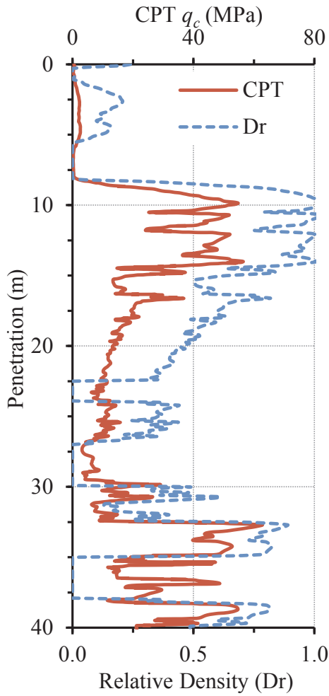
Fig. 6. Site CPT q_c and Relative Density ( D_r ) Profiles. (a) Caravel
