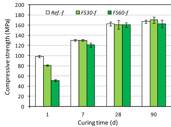
Fig. 8. Compressive strength of fiber-reinforced UHPC mixtures.
