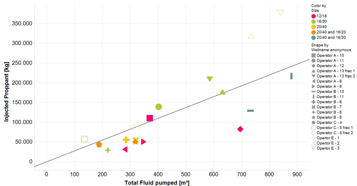
Figure C.10: The concentration of proppant in the pumped fluid. The black dashed line is roughly indicating the average concentration and is almost equally to figure C.5: 275 kg proppant per m³ fluid. Since the amount of pumped proppant is much higher compared to the wells that are fractured later in production life, the total fluid pumped is also much higher.
