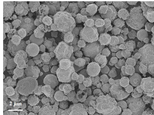
Figure 8. SEM photo of Cu@Ag particles
