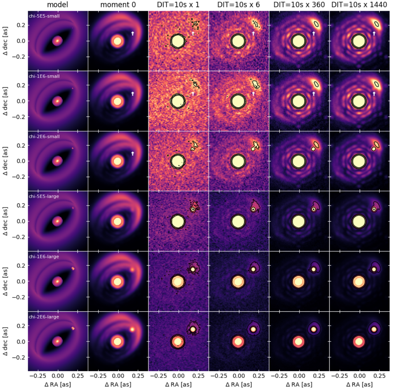
Fig. 5. Synthetic channel maps of v(1-0)P08 line ( 4.73587\ \mu\text{m} ) from the CPDs of varying physical extent and background irradiation. The CPD is placed at maximum elongation ( \theta = 90^\circ ). The leftmost column contains the input model at the extracted velocity ( +6.8\ \text{km s}^{-1} relative to the stellar reference frame). The asymmetry in the moment 0 map in column 2 is due to telluric contamination. The third to sixth columns include the synthetic channel maps for an increasing series of total detector integration times indicated at the top of each column. The black contours indicate a count value excess relative to the background of 25%, 50%, and 100%. The color range of each image has been logarithmically scaled with boundaries corresponding to the minimum and maximum values found outside of the central half of the stellar PSF. Where it is not apparent by eye the position of the CPD is indicated with a white vertical arrow. The six-fold symmetry apparent in longer integration times is a result of the ELT point spread function acting on the central star. The colormap normalization has been configured to maximize the visibility of the CPD.
