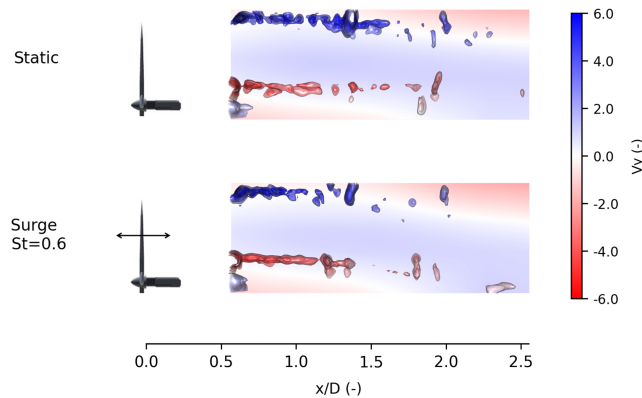
Figure 7. Swirling strength iso-surfaces coloured by vorticity, and streamwise velocity trend in the background for the vertical plane at y = 0 and downstream distance 0.6–2.5D. From top to bottom: static and surge St = 0.6 .
