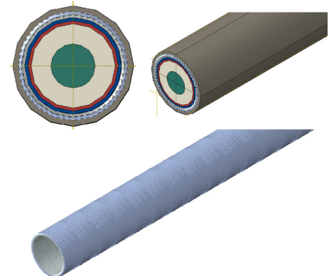
Fig. 8. Finite element model of the power cable.
