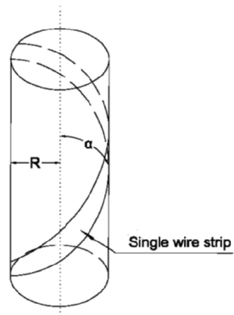
Fig. 4. Helical wires.
