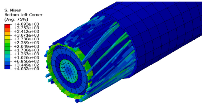
Fig. 25. The final Mises distribution of the cable under anti-clockwise torque.
