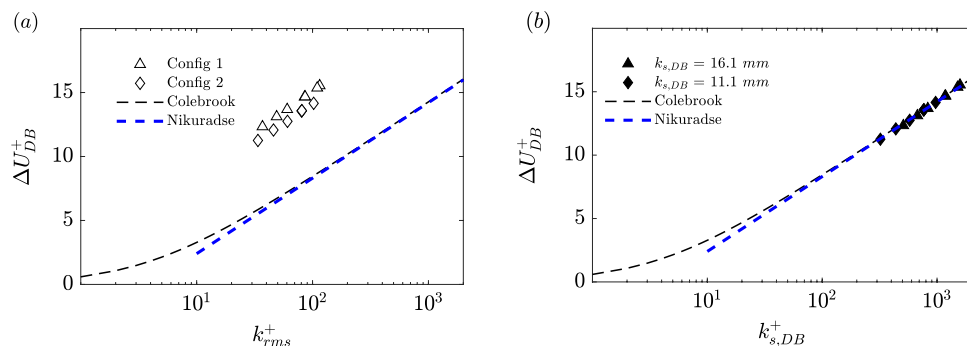
Fig. 2 a Variation of the roughness function \Delta U_{DB}^+ as a function k_{rms}^+ with \Delta U_{DB}^+ determined from drag balance measurements and boundary layer thickness, using equation (1.5). b Variation of \Delta U_{DB}^+ with respect to k_{s,DB}^+ determined using equation 7 with the constant
