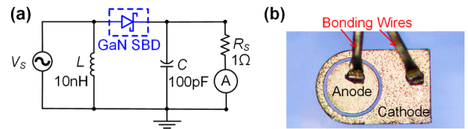
Figure 7. (a) Schematic of the microwave power detector with the GaN SBD. (b) Photograph of the GaN SBD with bonding wires.
