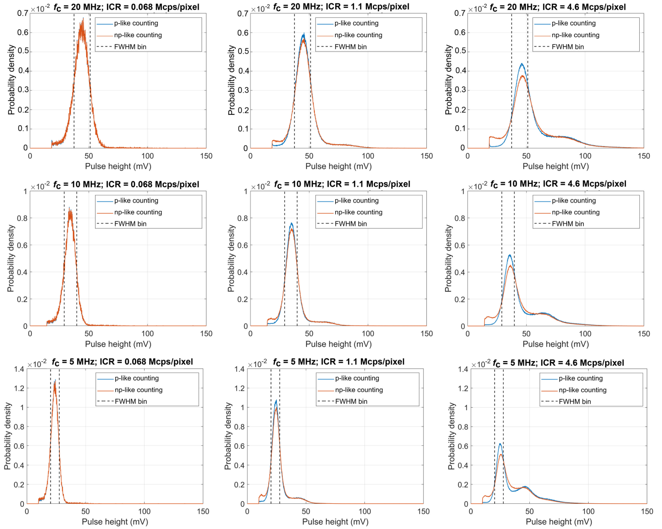
Fig. 9. Normalized pulse height spectra, which represent the probability that a registered count gets associated with a certain pulse height, measured with the LYSO:Ce detector and both the paralyzable-like and nonparalyzable-like counting algorithm. From left to right, the estimated input count rate is increasing. From top to bottom, the cut-off frequency f_c of the second-order low-pass filter applied to the raw pulse trains is decreasing. The FWHM bin, used to calculate the SDF [see Section II-D and (5)] is visualized by means of the vertical dashed lines.
