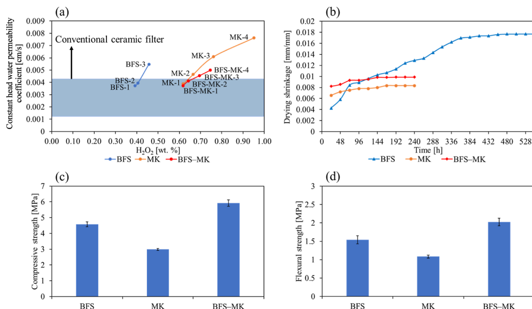
Figure 1. (a) Effect of the amount of H_2O_2 on the constant headwater permeability coefficient in AAFs. The targeted value of the coefficient is shown with the blue area in the figure; (b) comparison of length change in three different AAFs (BFS, MK, and BFS-MK) with time, (c) comparison of compressive strength (MPa), and (d) comparison of flexural strength (MPa).
