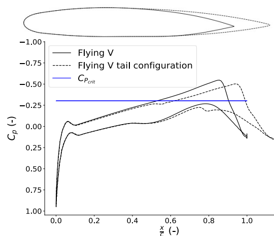
(b) Flying V, tail configuration root pressure distribution
