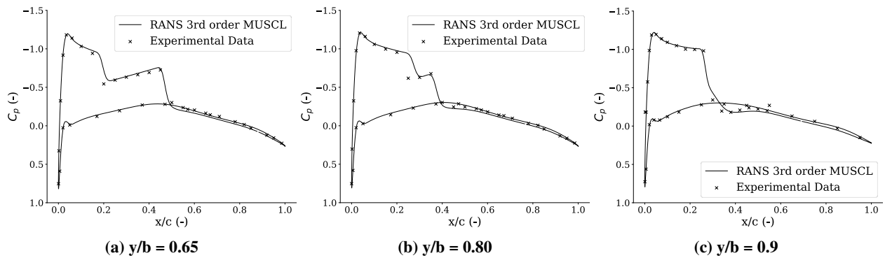
Fig. 11 Pressure distribution validation on the ONERA M6 wing (Mach = 0.8395, \alpha = 3.06^\circ , Re = 11.72 million)
