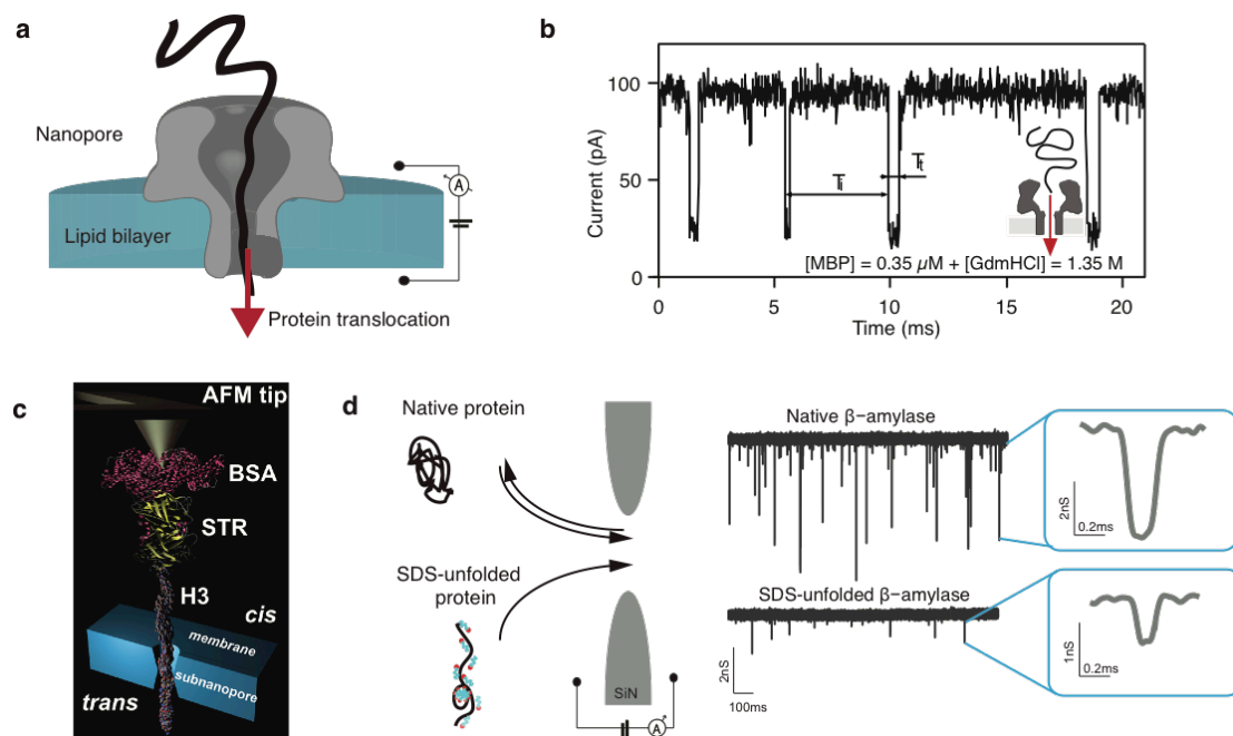
Figure 4. Translocation of peptides and unfolded proteins through nanopores. (a) Schematic representation of a biological nanopore set-up. (b) Representative current traces when GdnHCl was used for unfolding and translocation of a maltose binding protein through an alpha-hemolysin pore. (c) Schematic where a protein is immobilized at an AFM tip and translocated through a nanopore. (d) Schematic of native and SDS-unfolded protein translocation through a solid-state nanopore including typical current traces of native and SDS-unfolded proteins. Panel b from ref 78 ; panel c from ref 90 , and d from ref 77 .
