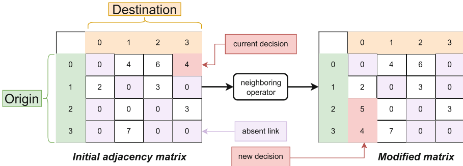
Fig. 3. Simulated annealing neighboring operator functioning. The operator modifies the current decision to a new decision according to three operations: adding, removing, and swapping.
