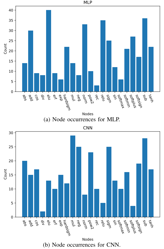
FIGURE 5. Function node occurrences in the evolved activation functions.
