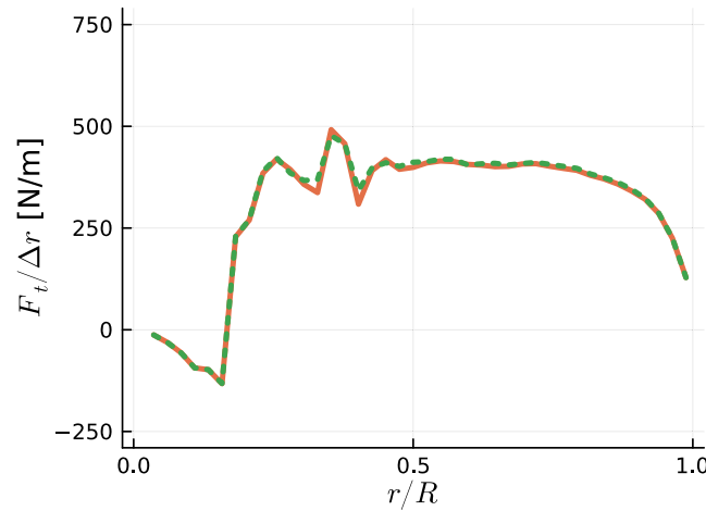
FIGURE 14 Tangential force per unit span over blade radius. AL-LBM rotor refined results as orange lines, AL-LBM blade refined results as green dotted lines.
