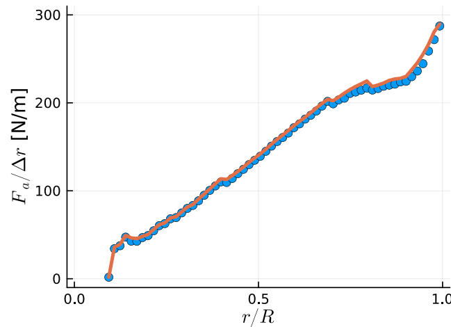
FIGURE 6 Axial force per unit span over blade radius. SOWFA results shown as blue circles, AL-LBM results as orange lines.
