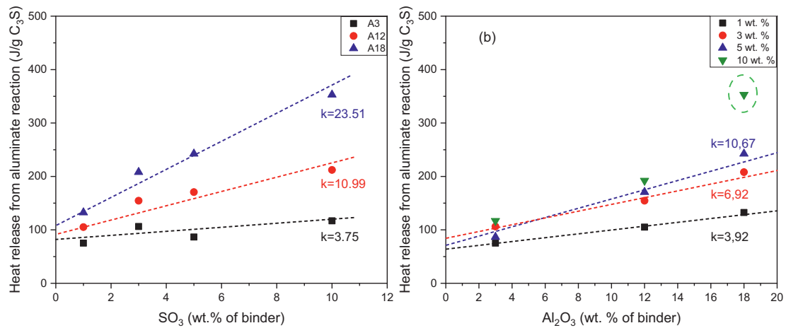
Fig. 9. Heat release from aluminate reaction against (a) \text{SO}_3 content of gypsum and (b) \text{Al}_2\text{O}_3 content of slag.
