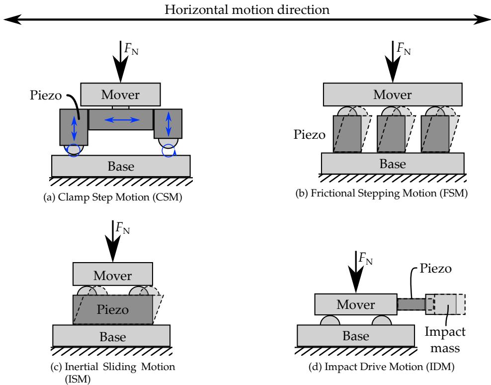
Figure 3.3.: The piezoelectricity based positioning concepts presented in [Wulp, 1997]. The concepts are presented in a simplified form that generates motion in the horizontal direction. The dashed lines indicate another stage in the motion cycle. The CSM and the FSM concepts in Figures 3.3a and 3.3b are in the piezo stepping category (Section 3.3.1). The ISM and IDM concepts in Figures 3.3c and 3.3d both use inertia and are in the piezo inertia category (Section 3.3.3).
