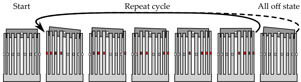
Figure 4.17.: One full tilt cycle that uses all fingers on a 16 finger TSA. The active heaters, that elongate their fingers, are indicated in red. The solid arrow indicates the fastest tilt cycle. The dashed arrow indicates a cycle that includes a state where all fingers are cold. This can be used to easily measure the current tilt angle for control purposes.
