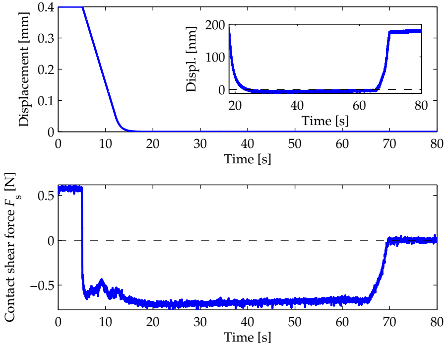
Figure 5.13.: An example of pre-sliding position control using a velocity-position control loop. The positioning goal (indicated by the dashed line) is 0 nm, while the initial position is 0.4 mm. The goal is achieved with a 10 nm error within 30 seconds, however a 180 nm error is introduced when the contact shear force is brought back to 0 (between 60 and 70 seconds). This displacement is shown in the inset graph.
