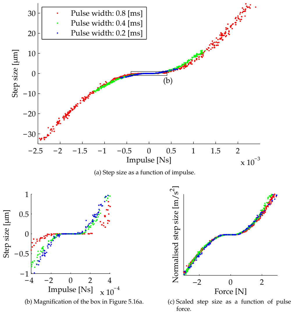
Figure 5.16.: The displacement step-size variation of force pulses of different force pulse amplitudes and pulse widths (Figure 5.16a). The current pulses are generated using a current amplifier and have a duration of 0.2, 0.4 and 0.8 ms. The force was limited to \pm 3 N. This experiment shows that the effective impulse determines the displacement magnitude. The bottom left graph (Figure 5.16b) is a magnification of the black box in the top graph and shows the differences in step size for small impulse. The bottom right graph (Figure 5.16c) is scaled to show that the force (on the x-axis), and not the impulse, determines whether the contact displaces.
