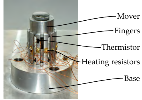
(b) The first circular TSA prototype built by Jeroen van Schieveen. The base and fingers of this actuator are monolithic. The 12 fingers are heated in pairs opposite to each other.
