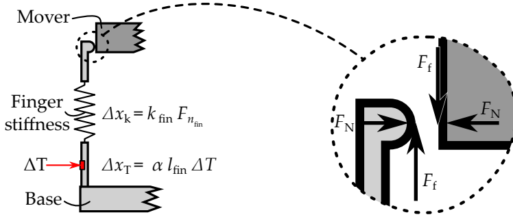
Figure B.2.: Mechanical model overview
