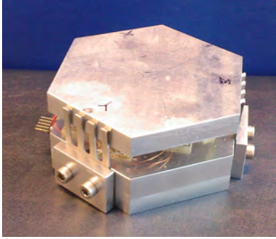
(a) The three sided thermal actuator configuration with 3 times 4 fingers, as described in [Schieveen and Spronck, 2009], built by Jeroen van Schieveen and Ruimin Yang.
