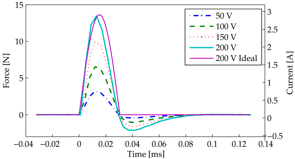
Figure 5.15.: Typical force (left scale) and current (right scale) profile in time of an electromagnetic force pulse generated using the current pulse generator circuit shown in Figure 5.14. The current is measured using a current probe at a sample frequency of 250 kHz. The force is derived from the current measurement. Comparing the 200 V pulse with the ideal (sinusoidal) pulse shape, the measured reverse current after the pulse becomes clear. This is caused by the non-ideal properties of components in the pulse generator circuit.
