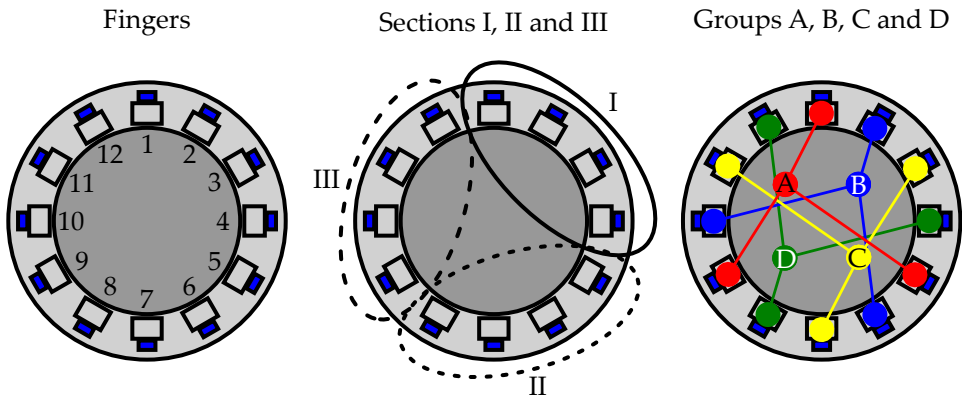
(a) Thermal Slider Actuator: the number of fingers, sections and groups are: n_f = 12 , n_s = 3 and n_g = 4 .
