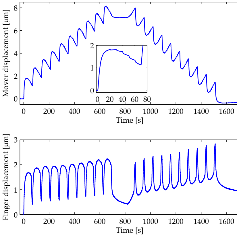
Figure 4.15.: Measurement of the displacement of the mover and one of the 12 fingers with respect to the base of the TSA during 10 upward and 10 downward cycles. The inset graph shows a detail of the mover displacement of the first upward cycle. A comparison of this measurement with a numerical model of this TSA can be found in Appendix D.
