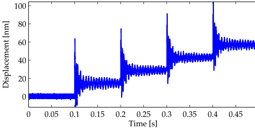
Figure 5.18.: Measured displacement during a series of 4, 4.5 N peak, 0.03 ms electromagnetic force pulses, resulting in results in a 15 nm net displacement with 50 nm overshoot.
