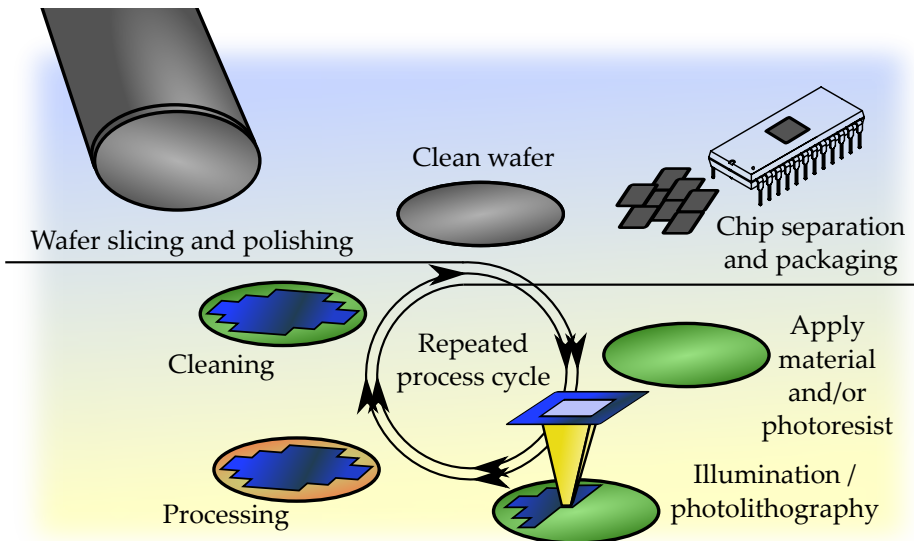
Figure 1.2.: The Integrated Circuit (IC) manufacturing cycle, schematically depicted. Inspired on [Munnig Schmidt et al., 2014].
