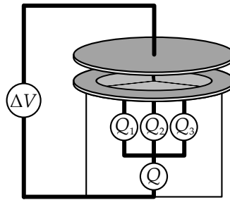
Figure 2.8.: Schematic representation of a segmented electrode with a guard ring that can be used to measure both the electrode distance and the tilt angle.
