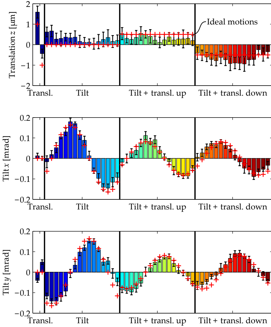
Figure 4.22.: Measured (parasitic) motion and repeatability of the 16 finger TSA in 50 selected directions. A bar in a colour represents the mean displacement due to a step-cycle (vertical axes). The cycles are grouped (horizontal axes) according to their intended motion: Translation, Tilt, Tilt and translation upward and Tilt and translation downward. The three different graphs indicate the three displacement components, one translation and two tilt directions. The black bars indicate the standard deviation \sigma . The directions of x , y , and z are defined in Figure 4.14. The cycles shown here use a time-step dt of 10 seconds and tilt sections of 7 fingers. The red plus signs (+) indicate the motions that are expected based on an idealised model. The cycles were performed in a random order and 0.24 W was supplied per finger.
