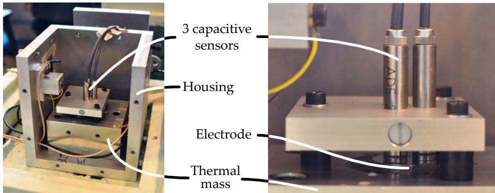
Figure C.3.: Pictures of the capacitive measurement set-up. On the left the aluminium housing and the block that contains the actuator. On the right a detail of the capacitive displacement sensors on top of the mover (in this case a steel electrode) that is clamped by the actuator. The sensors are placed on a circle of 13 mm diameter. The aluminium box was closed on all sides during measurements to reduce the influence of labs temperature variations.
