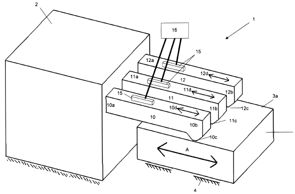
Figure 4.1.: The schematic illustration of the working principle of the Thermal Slider Actuator as depicted in the TSA patent [Schieven and Spronck, 2009]. It shows a base (2), a mover (3) and three thermally actuated fingers (10, 11 and 12).
