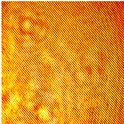
(a) Interferogram of which position and tilt are extracted, captured with the camera and set-up shown in Figure C.1. An initial tilt angle in the reference mirror causes the visible fringes (the sloped line pattern). Deviations in horizontal and vertical frequency correspond to tilt motion, whereas an overall phase change corresponds to a translational motion.
