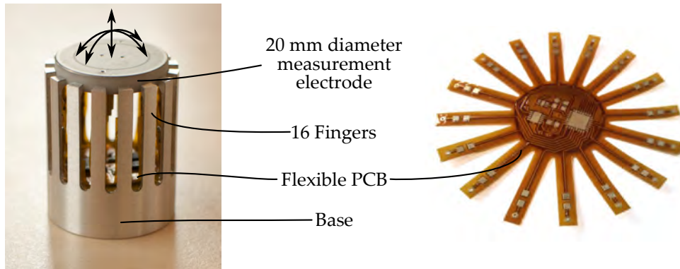
Figure 4.5.: The 16 finger TSA with integrated electronics as designed and made by Jeroen van Schieveen. The heating resistors are mounted on a flexible PCB, which in turn is glued on the inside of the stepper base. In the centre the PCB contains a microprocessor and a power switch/multiplexer, so that only power and serial data has to be provided externally, for instance over a USB connection.
