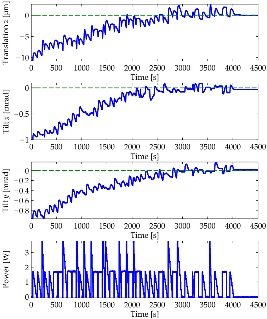
Figure 4.26.: Measurement of three DoF position control of the 16 finger TSA. The positioning target is zero translation ( z ) and zero tilt in both x and y directions, indicated by the dashed green lines. The initial position error is 10.8 \mu\text{m} in translation and 1.4 \text{ mrad} in tilt. The final positioning error is 0.15 \mu\text{m} in translation and 30 \mu\text{rad} in tilt direction. The bottom graph shows the total heating power of the actuator. Fine positioning starts after approximately 3000 seconds, as can be seen from the pauses between the cycles.
