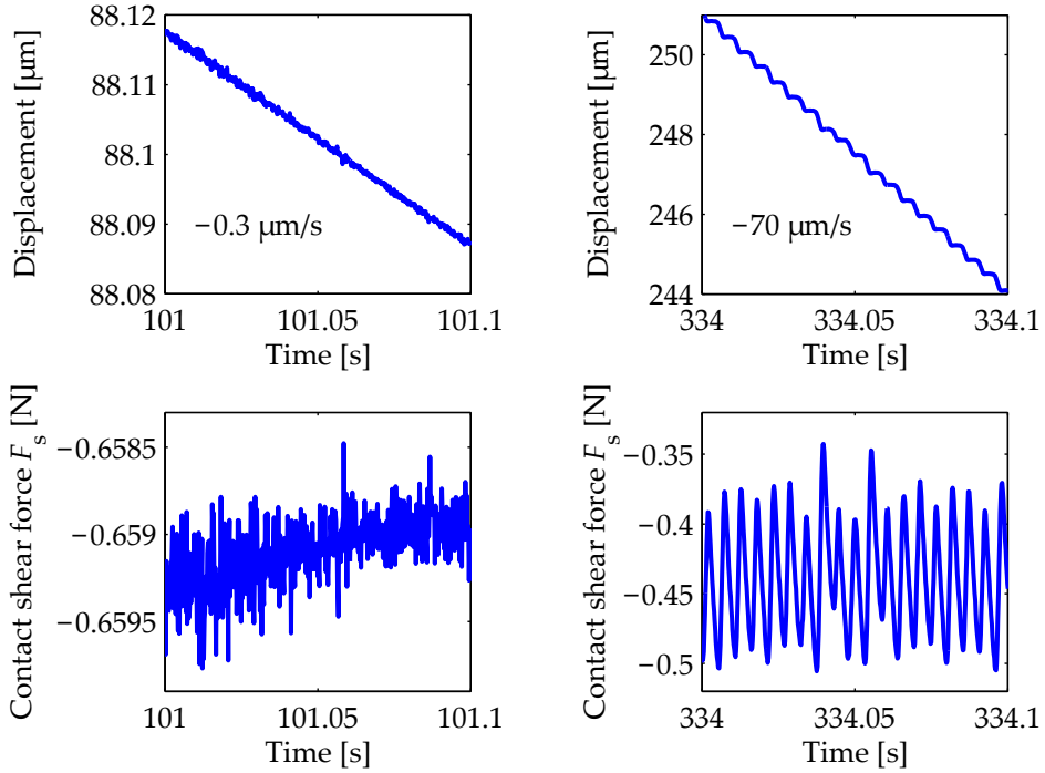
Figure 5.10.: Pre-sliding motion of a steel friction contact at two motion velocities. This measurement is performed using the closed loop velocity controller shown in Figure 5.8. At -0.3 \mu\text{m/s} , the force variation is minimal and the velocity is constant. (This confirms that the displacement is non-elastic.) At -70 \mu\text{m/s} the contact cycles between the stable and the unstable region and therefore shows a significant force and velocity variation.
