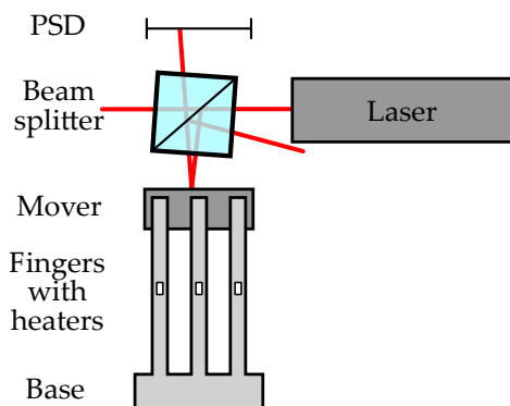
Figure C.4.: Angle measurement using a 2 dimensional PSD (Position Sensitive Detector). The actuator is mounted similarly to the interferometric set-up shown in Figure C.1. The tilt angle is determined from the position of the laser spot on the PSD.
