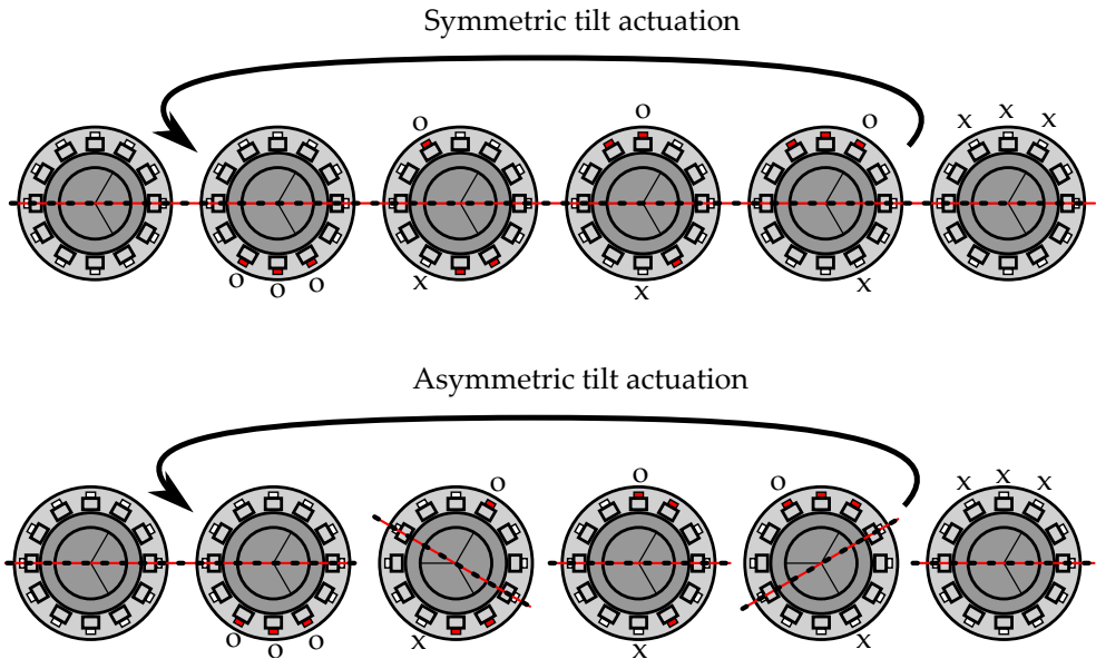
Figure 4.18.: Symmetric and asymmetric tilt actuation. The active heaters are indicated in red and at each cycle step an 'o' indicates switching on, an 'x' indicates switching off. The asymmetric tilt cycle results in parasitic tilt motion (in the other tilt direction) during the cycle, as the fingers that are moving up and downward (heating and cooling respectively) apply a friction torque with respect to the indicated symmetry axes (red and dashed lines).
