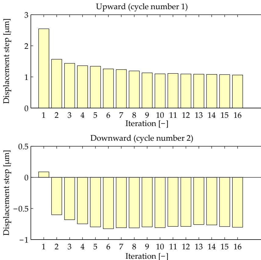
Figure 4.23.: Convergence of consecutive translation cycles with 4 sections of 4 groups on a 16 finger TSA. The top graph shows a series in upward direction, the bottom graph in downward direction. Both cycle series were executed from room temperature and from arbitrary initial contact conditions. The convergence effects from the initial pre-load and thermal condition are visible (iteration 1-8), as well as the friction direction dependency (iteration 9-16). Note however that the initial conditions in this experiment are not necessarily representative for operational conditions. A heating power of 0.24 W was supplied per finger.
