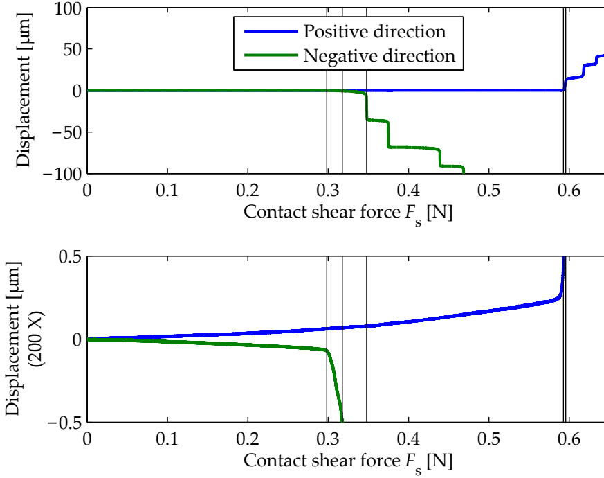
Figure 5.5.: Micrometre scale displacement response of a clean steel-steel friction contact to a contact shear force ( F_s ) increase from 0 to 0.7 N in 65 seconds. The force at which the contact starts moving plastically varies significantly due to local conditions and history. This experiment shows that although there are strong non-linearities in the friction behaviour, the displacement is always gradual. The black vertical lines in the graph indicate displacement time instants in the graphs at both magnifications. They show that at different displacement scales, different effects are visible. The variation in the absolute shear pre-load between the experiments is smaller than 10 mN. The normal force ( F_N ) equals 1.7 N.
