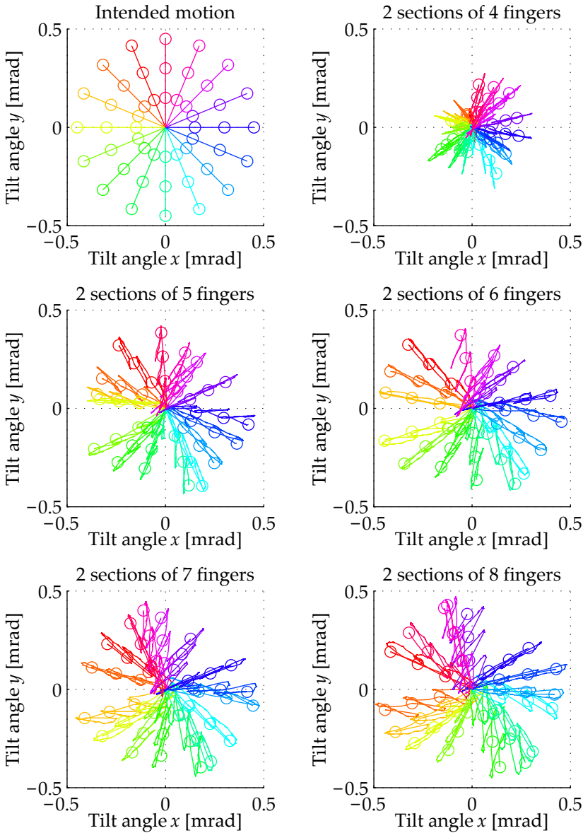
Figure 4.21.: The intended tilt displacement (top-left graph) of the 16 finger TSA compared to those measured using the capacitive 3 DoF measurement set-up. The number of fingers that was used for tilt actuation was varied in the measurements, so that the influence on the tilt motion is shown. As was already shown in Figure 4.20, only significant tilt displacements occur when more than four fingers are used. Also, when the measured motions are compared to the ideal directions, both deviations of the end-points (the circles) and within the motion (the line between the circles) become apparent.
