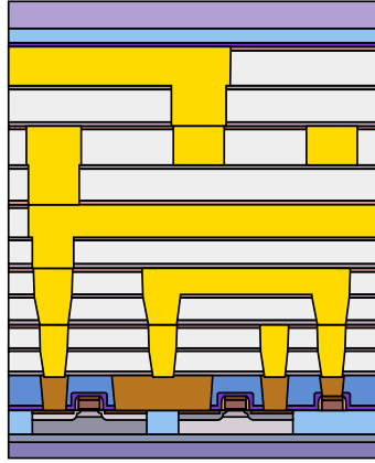
Figure 1.1.: Illustration of the layered structure of an integrated circuit. (This image is based on the work of Cepheiden.)
