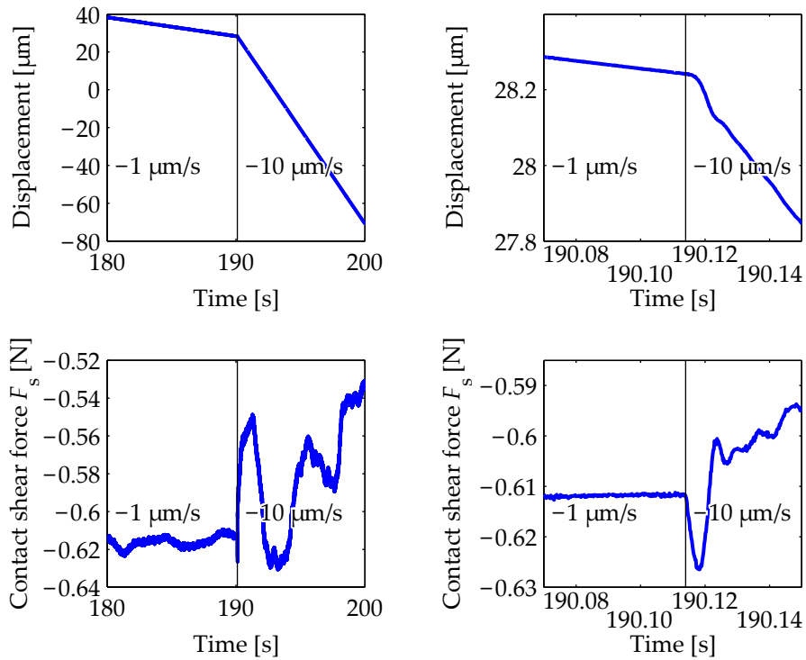
Figure 5.9.: Transient behaviour of a velocity controlled friction contact at a change of the velocity set-point from -1 to -10 \mu\text{m/s} . On the left a velocity change is shown on a 20 seconds scale. The graphs on the right show the same data zoomed in on the velocity set-point change.
