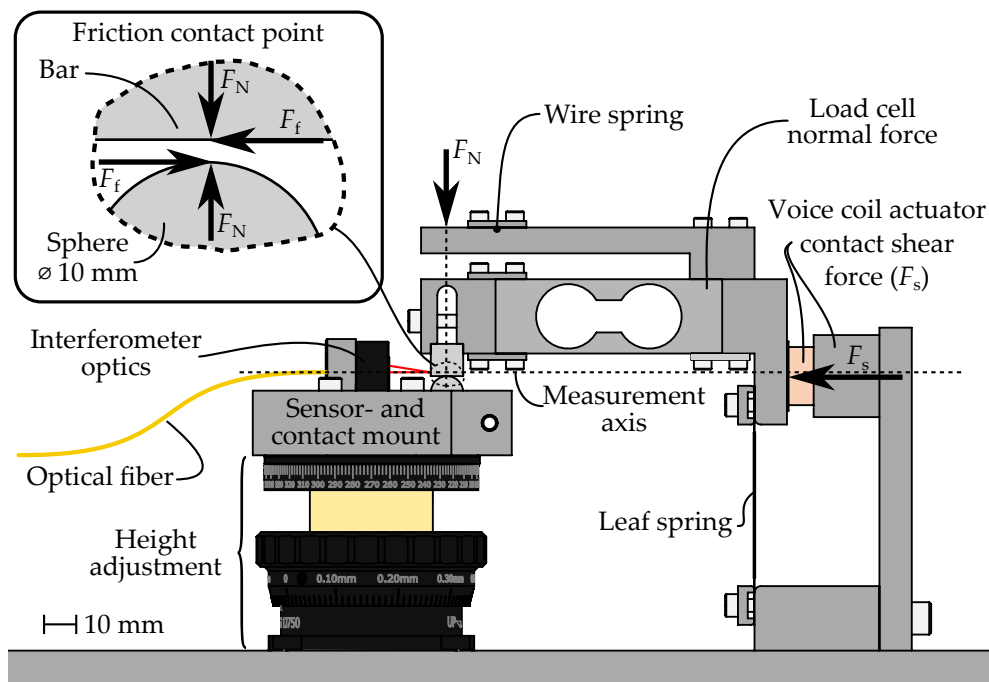
Figure 5.3.: Schematic drawing of the single point friction measurement set-up. The friction contact is as much as possible in line with the shear force actuator and the displacement measurement. The normal force is applied orthogonal to this line. A picture of the set-up is shown in Figure 5.4.
