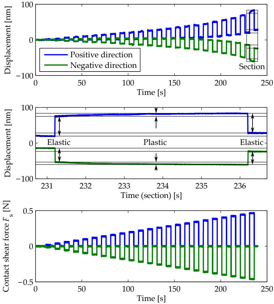
Figure 5.7.: Continuous pre-sliding shown by means of force step responses. The force increment of each step is 20 mN as is shown in the bottom graph. The middle graph shows both the elastic and the plastic part of the pre-sliding displacement of the last step-response, indicated with a black box in the top graph. The plastic displacement of the last steps is 8 \pm 1 nm. This experiment shows that plastic (permanent) displacement can be generated by applying a predefined constant contact shear force. A further increase of the contact shear force leads to unstable sliding.
