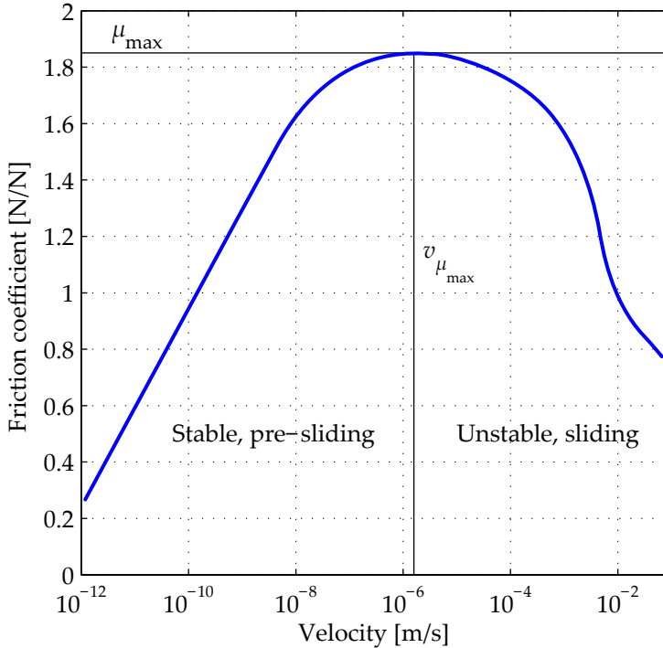
Figure 5.1.: Graph that qualitatively shows the maximum in the \mu(v) relationship, based on the steel-indium graph presented in [Burwell and Rabinowicz, 1953]. This relationship is valid for steady state velocities on this specific material combination. Literature and experimental results in this thesis however indicate that the shape of this relationship is more universally valid, for instance for steel-steel and aluminium-steel combinations. For these other materials it is likely that the maximum force is achieved at significantly lower velocities. The maximum in this graph ( \mu_{\max} ) is generally considered to be the static friction coefficient \mu_s , however, this relationship shows that a continuous motion also occurs at lower shear force levels.
