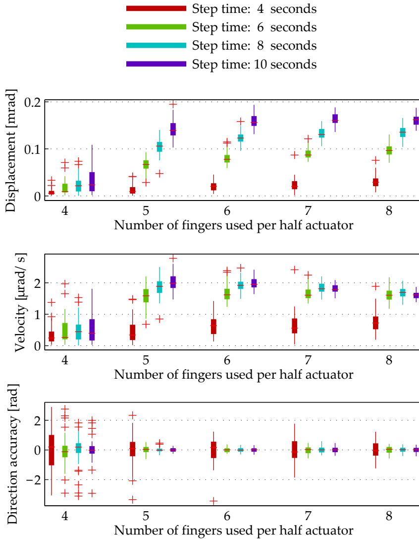
Figure 4.20.: Measurement results that show the influence of the number of fingers used for a tilt motion and the time steps on the motion step size and speed and the direction accuracy on a 16 finger TSA. The number of fingers mentioned in the diagram is the number of fingers that is used in a tilt-section each half of the 16-finger thermal slider actuator (Figure 4.5). Multiple tilt-cycles in 16 tilt-directions are taken into account. A 4 seconds step time or 4 step fingers lead to a relatively large variation on the tilt step size and motion direction. Longer step times and the use of more fingers do increase the step size, but not necessarily the average velocity. This measurement was performed using the PSD measurement set-up, as described in Appendix C.
