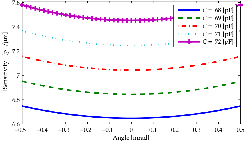
(a) Sensitivity as a function of the capacitance and the tilt angle. On each line the capacitance is constant, which means that for an increasing tilt angle \theta , the electrode gap x increases. For instance at 70 pF, the distance increases from 9.9 \mu\text{m} to 10.1 \mu\text{m} between 0 and 0.5 mrad. Note that the sensitivity variation is significantly smaller than for a constant gap distance as is shown in Figure 2.6b.
