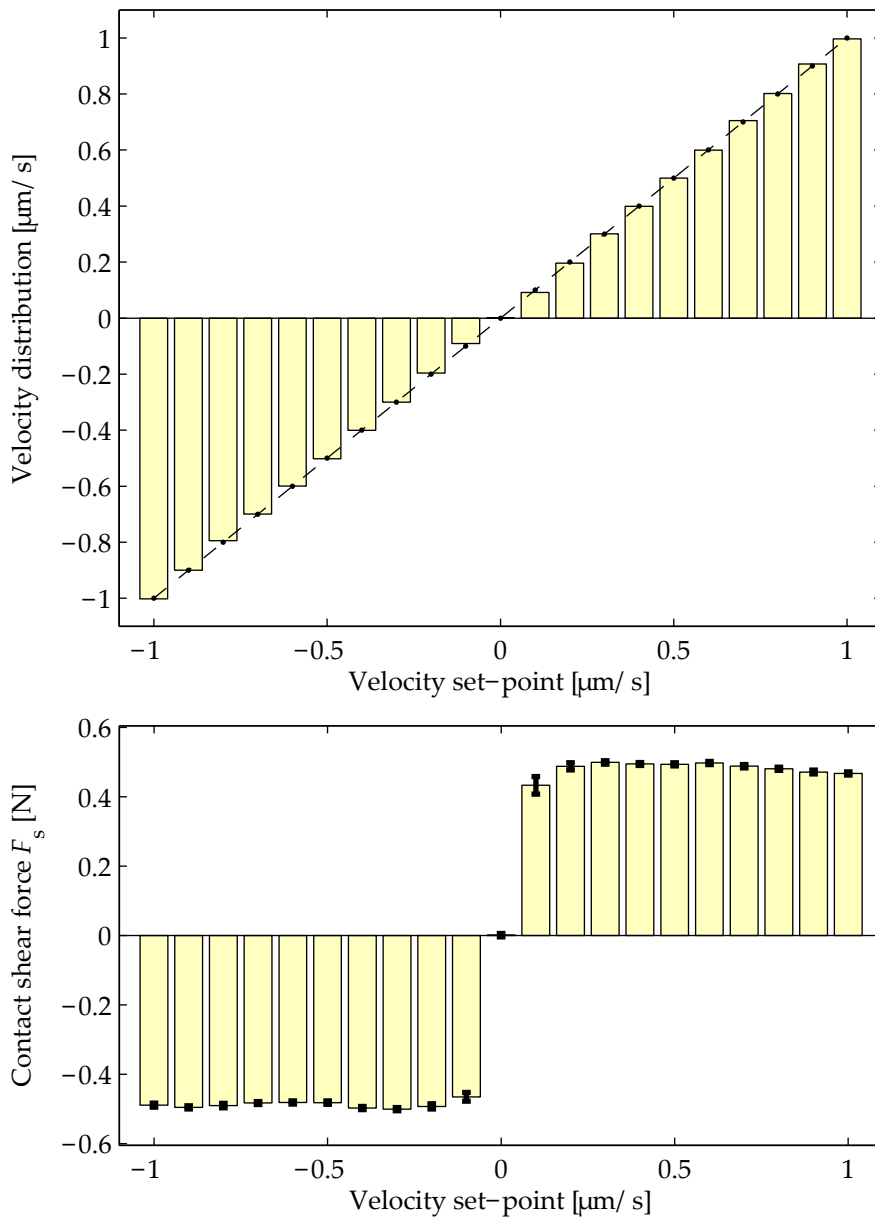
Figure 5.11.: Velocity control over a \pm 1 \mu\text{m/s} velocity range. The bars show the velocity and shear force at each set-point, recorded over approximately 10 seconds. The standard deviation of the velocity signal is constant and 5 \mu\text{m/s} in this range. It is omitted in the graph for clarity. The dashed line/dots in the top, velocity graph indicate the velocity set-points. The mean velocity error is always smaller than 10%. The bottom graph shows the mean contact shear force for each velocity and its standard deviation. This force is approximately constant at velocities above 0.1 \mu\text{m/s} .
