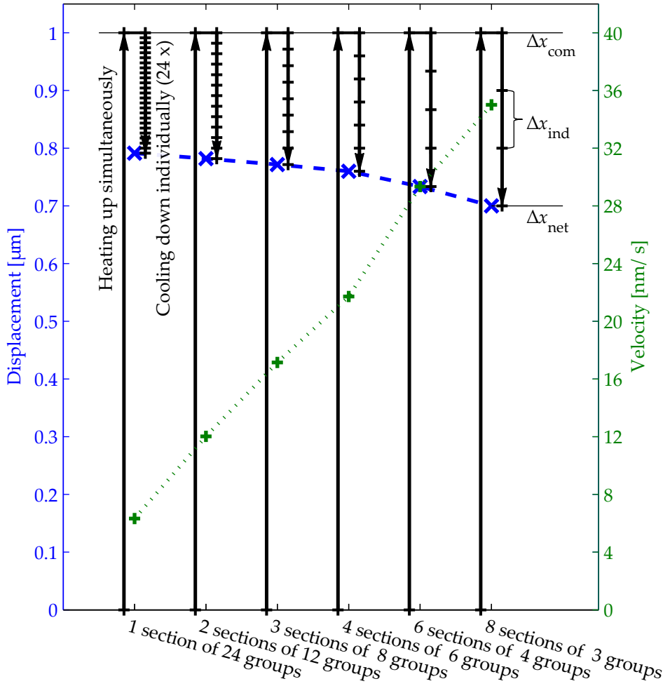
Figure 4.10.: Analytic approximation of grouping of a TSA with 24 fingers, where F_{f,\max} = F_N \mu_s = 1 \text{ N} , k_{\text{fin}} = 10^7 \text{ N/m} and \Delta x_0 = 1 \mu\text{m} (see (4.2)). The different grouping options are indicated on the horizontal axis. Each set of arrows in the graph indicates the motion of the mover of the TSA during one upward cycle. The displacement starts at zero and increases to 1 \mu\text{m} , according to Equation (4.2). Then, when individual groups of fingers cool down the mover moves along as is indicated by the downward arrow. The number of markings in the downward arrow and the magnitude of these steps is dependent on the number of groups that is used, as is described in Equation (4.6). The net displacement is indicated with blue crosses at the end of an arrow. Using less groups leads to a larger net displacement, but because each sub-step takes the same time, a smaller number of sub-steps leads to an increased motion velocity, as is indicated with the green + signs and on the right axis. The displacements that were indicated in Figures 4.3 and (4.8) are also shown at the arrows on the right.
