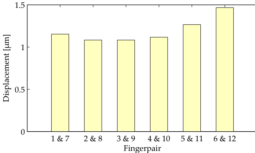
Figure 4.29.: Displacement of the mover of the TSA due to heating of a single pair of fingers. The difference between the finger pairs can be explained by the unequal clamping forces such as shown in Figure 4.30. This effect is measured on an ASML/PI-stepper such as shown in Figure 4.12, although a different TSA sample was used in this measurement.
