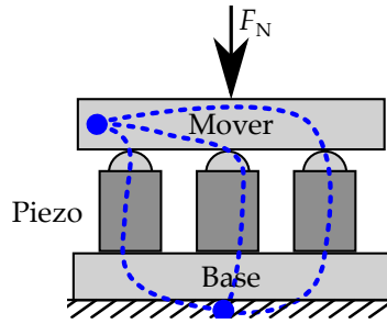
Figure 3.4.: Stability paths of the FSM actuator (see also Section 3.3.1 and Figure 3.3b). The blue dashed line indicates the stability path from an arbitrary point on the fixed world to an arbitrary point on the mover. The paths indicate that the base, the piezos, the contacts and the mover contribute to the stability of the mover.
