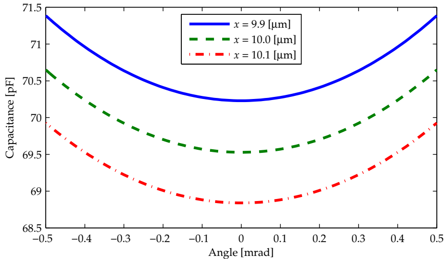
(a) Capacitance as a function of the tilt angle \theta , for three electrode centre distances x . Electrode tilt increases the capacitance, so that the apparent electrode distance is smaller. The capacitance is approximately 2% larger at an angle \theta of 0.5 mrad compared to zero.
