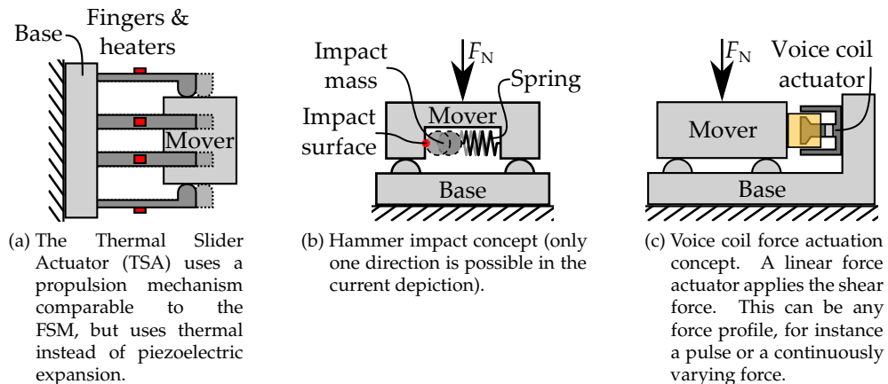
Figure 3.5.: Actuation concepts that use other forms of propulsion. These concepts can be derived from the piezoelectrically driven actuator concepts shown in Figure 3.3. A more detailed description of these concepts can be found in Sections 3.3.2, 3.3.4 and 3.3.5.
