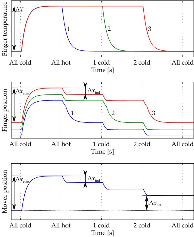
Figure 4.3.: Simulated temperatures and displacements of a 3 finger TSA. The thermal model consists of three elements, one for each finger, and the friction is modelled with only a static friction coefficient. The different lines in the two top graphs indicate the temperature and position changes of the different fingers in the TSA, also a finger number is shown. This simulation represents the behaviour of the simplified actuator shown in Figure 4.2. The step size \Delta x_{net} and the intermediate displacements \Delta x_{com} and \Delta x_{ind} are defined in Section 4.2.2.
