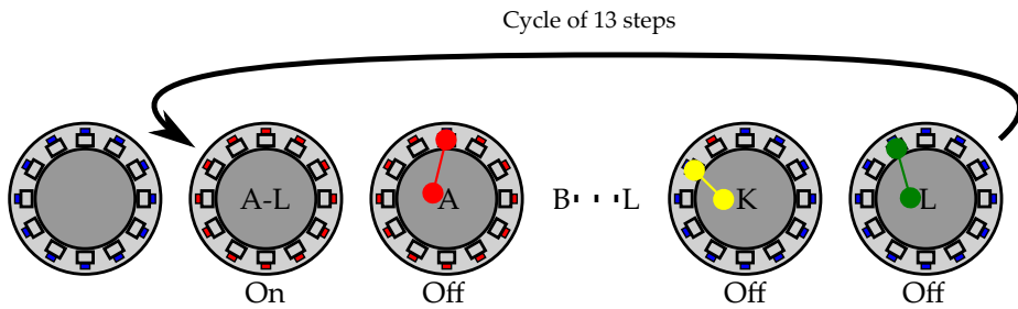
(b) Grouped in 1 section and 12 groups (A to L): n_s = 1 and n_f = n_g = 12 .
