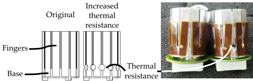
Figure 4.27.: Illustration of a method to increase the thermal resistance between the fingers and the base, applied on a ASML/PI TSA. The picture on the left schematically shows the difference between the original and the adapted actuator, the photograph on the right shows the realised parts (the housing shown in Figure 4.12 was omitted). The modification consists of a width reduction of all fingers close to the base. The thermal effect of this modification is shown in Figure 4.28
