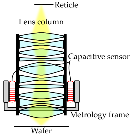
Figure 1.5.: Schematic representation of the lens column system and the metrology frame in which both the lens and the two sensor systems are suspended.
