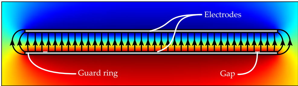
(b) Electric field and potential of a parallel plate capacitor with a guard ring.
