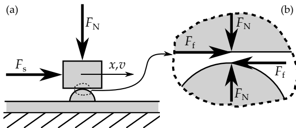
Figure 3.2.: Definitions of the friction contact. Two forces act on the mover: normal force F_N , and shear force F_s , indicated on the left side (a). This results in an internal friction shear force F_f , which under stationary conditions equal to F_s . The friction shear force is indicated on the right (b). For clarity the two contacting bodies are separated. The mover and the contact have a relative displacement x and velocity v .
