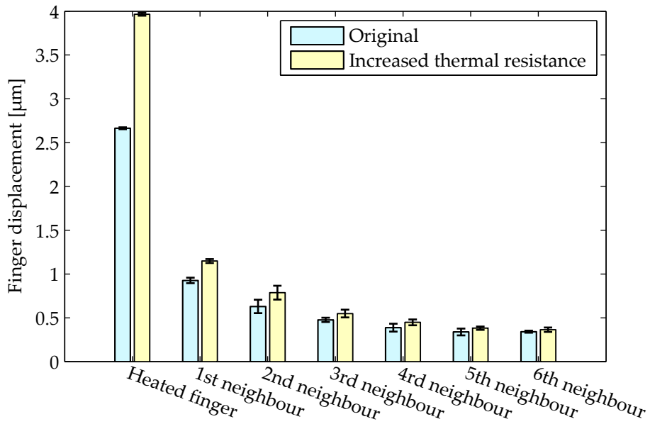
Figure 4.28.: Measurement of the thermal crosstalk between fingers of the ASML/PI TSA for a heating period of 60 seconds. The influence of increasing the thermal resistance between the fingers and the base, see Figure 4.27, is shown. The heated finger of the adapted TSA has a thermal expansion that is approximately 1.5 times larger than the original. The expansion of the first neighbour is only 1.2 times larger. The thermal cross-coupling is therefore significantly reduced.
