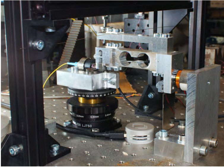
Figure 5.4.: Picture of the single point friction measurement set-up. This set-up is schematically shown in Figure 5.3.
