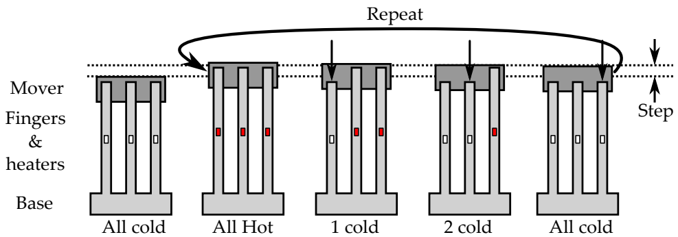
Figure 4.2.: The working principle of a single motion direction Thermal Slider Actuator (TSA) shown on a simplified actuator with the theoretical minimum number of 3 fingers. The upward motion is demonstrated. First all fingers heat up, displacing the mover. When a single finger cools down, it will slide over the electrode surface due to the thermally induced preload, while the electrode is clamped by the other fingers. An arrow indicates the relative motion of the finger with respect to the mover. When all fingers have subsequently cooled down passively, a net displacement of the mover remains. Thermal cycle order can be inverted to achieve a single-dimensional downwards movement. The resistors indicated in red are heating their finger.
