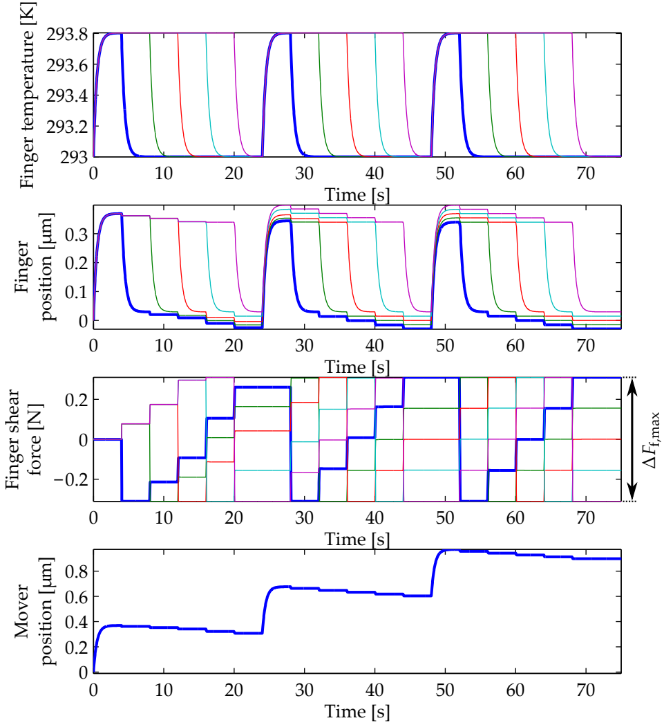
Figure 4.9.: Simulation of three TSA cycles on a 10 finger actuator. It started at zero contact shear force, as is show in the third graph at time equals 0. After the second iteration (at 45 s) the forces follow a stationary pattern, where the contact shear forces are always equally distributed between -F_{f,\max} and F_{f,\max} , where is in this case \Delta F_{f,\max} = 2F_{f,\max} = 0.6 N. For clarity the temperature, shear force and position of the first finger is indicated with a thicker line.
