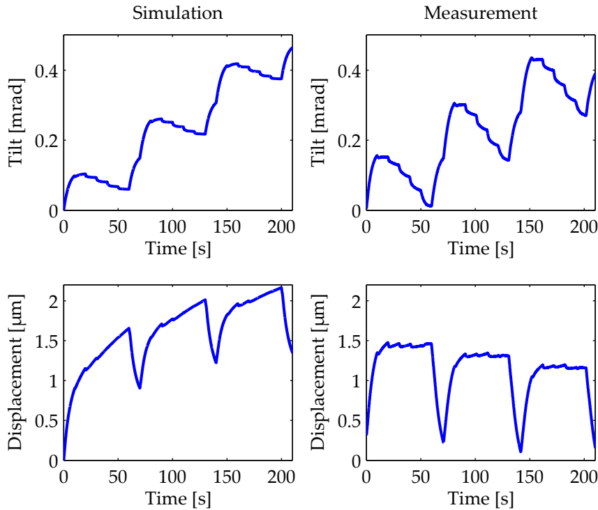
Figure 4.19.: Simulation (left graphs) and measurement (right graphs) results of tilt actuation on TSA with 16 fingers using 2 times 5 fingers for tilt actuation. Positions in micrometres and tilt angles in milliradians. A tilt cycle is performed three times with an all-off state in between (the cycle indicated with a dashed arrow in Figure 4.17). This effect is clearly visible in the dip in the bottom (displacement) graphs. The top (tilt) graphs show a typical tilt motion. The (parasitic) motion in the displacement direction (bottom graphs) can be explained by overall heating of the system (simulation) and by actuator non-uniformities that also cause remanent translations (measurement). This measurement is performed on the 16 finger TSA (Figure 4.5) using the 3-DoF capacitive measurement set up described in Appendix C. A comparison of the measured TSA translational motion with this model can be found in Appendix D.
