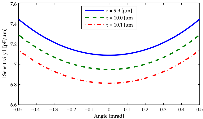
(b) Absolute value of the sensitivity in x -direction as a function of the tilt angle \theta , for three distances x . The sensitivity is approximately 5% larger at an angle \theta of 0.5 mrad compared to zero.
