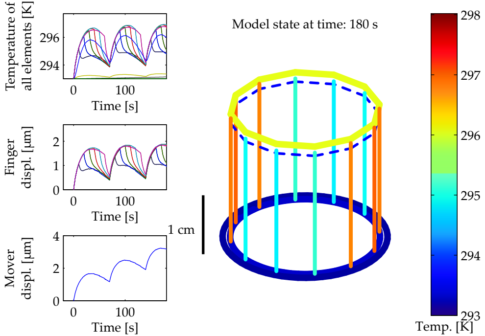
Figure B.4.: Graphical representation of a 12 finger TSA model. On the left side of this figure three separate graphs of respectively the temperatures of all elements in the model (the fingers, the mover, the base and the plate, see Figure B.1), the displacement of the fingers and the displacement of the mover are shown. The schematic drawing in the centre shows the temperatures and deformation of the parts of the TSA, the colours represent their temperatures. Compare this graphic for reference to the picture of a TSA demonstrator in Figure B.3. The blue, dashed ring represents the initial location of the mover. All initial temperatures are 293 K and all displacements are scaled by a factor 500 in the drawing. In the current state, 6 fingers are heated (shown in orange/red, around 297 K). A thermal cycle with 2 sections and 6 groups is used (see Section 4.2 for details on grouping).
