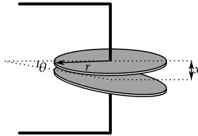
Figure 2.4.: Circular plate capacitor with tilted plates. The parameters are distance x , radius r and relative angle \theta .
