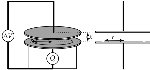
(a) Schematic representation of a parallel plate capacitor with guard ring (bottom electrode).
