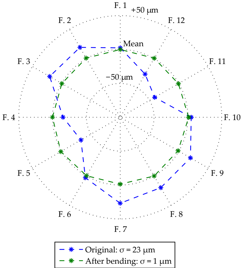
Figure 4.30.: Radial deviations of the neutral position of the fingers of a TSA. These measurements on an ASML/PI-stepper show the position deviations with respect to their mean value. The normal force variation that is associated with the deviation of the original actuator is more than 0.5 N. The measurements for the same actuator after manual correction (plastic deformation) are shown in green.
