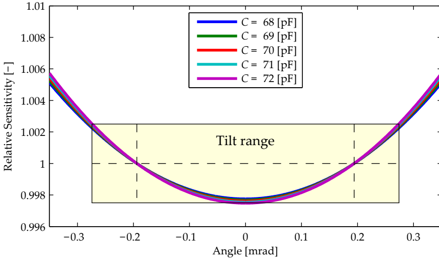
(b) Relative sensitivity as a function of the capacitance and the tilt angle. The reference value, indicated with the dashed lines, is chosen such that the sensitivity error remains within \pm 0.25\% . This results in a \pm 0.27 mrad tilt range.
