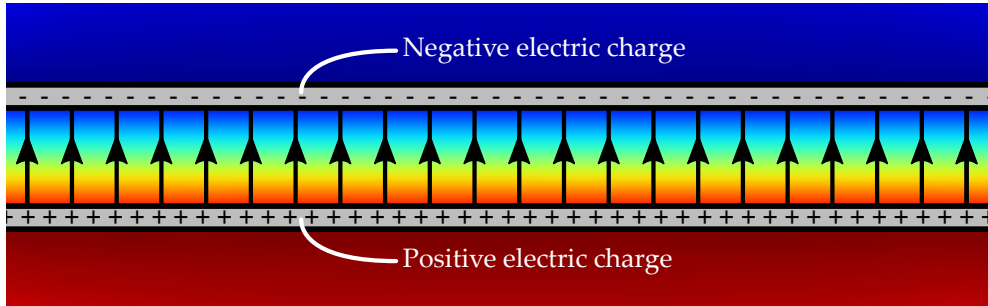
Figure 2.2.: Illustration of the electric field of a pair of charged infinite parallel plates. The electric field is only non-zero between the plates, as is indicated with the arrows. The colours in the picture indicated the electric potential from high (red) to low (blue).
