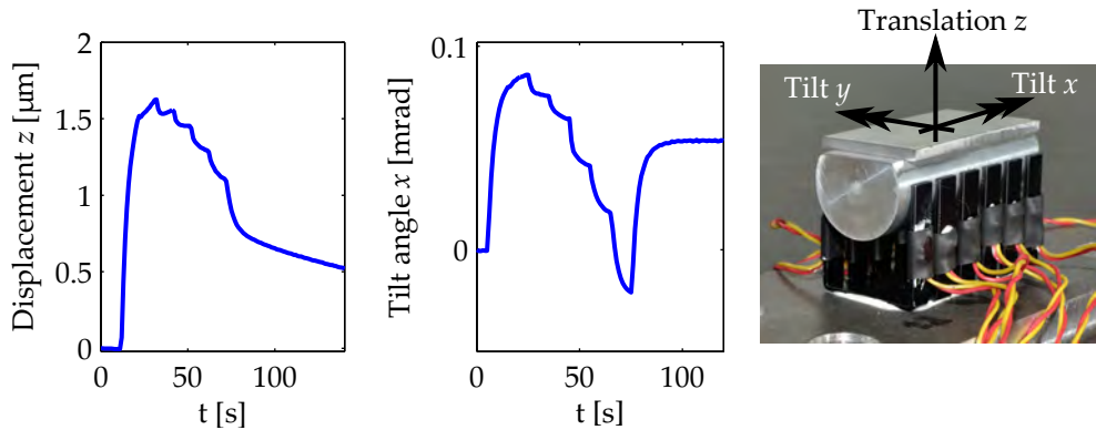
Figure 4.31.: A typical translation ( z ) and tilt ( x ) step (not measured simultaneously) of the simplified thermal slider design that was introduced in Figure 4.13. Tilt around the y -axis is relatively ineffective on this actuator due to the location of the fingers.
