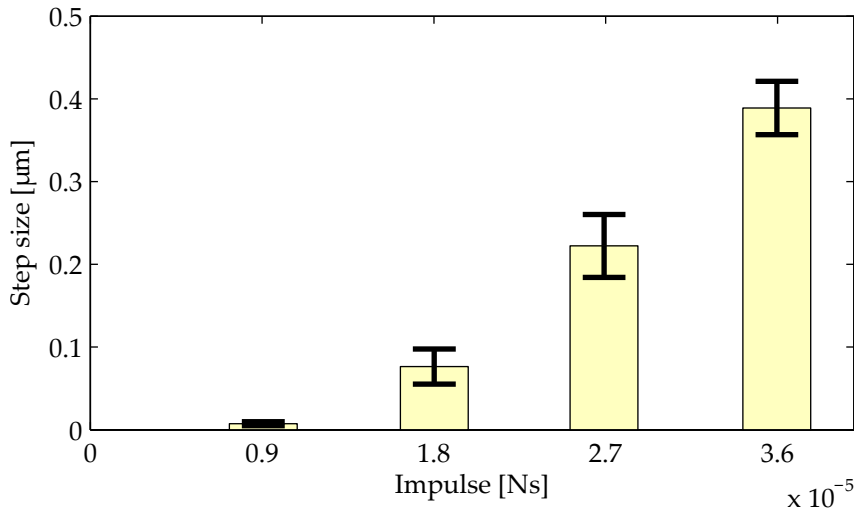
Figure 5.19.: Displacement due to short electromagnetic force pulses. The current pulses were generated using a dedicated current-pulse circuit (see Figure 5.14) and have a duration of 0.03 ms. The mean displacement step and its standard deviation during a single sequence of 180 steps is shown. The smallest step-size is 7 nm with a 2 nm standard deviation.
