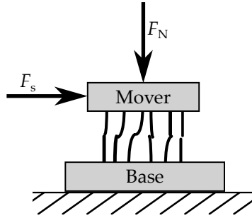
Figure 5.2.: Illustration of an asperity or bristle model of a friction contact. This can be seen as a more detailed view of Figure 3.2.
