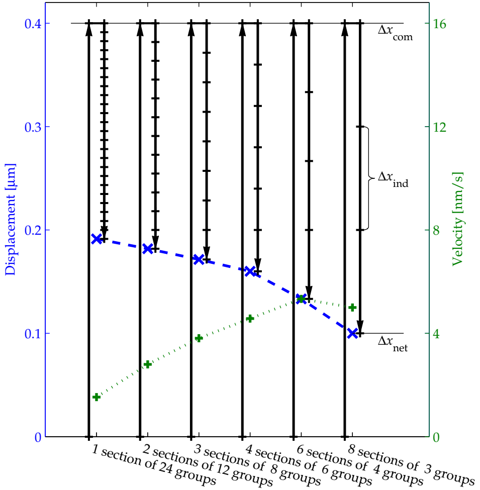
Figure 4.11.: Analytic approximation of grouping of a TSA as was shown in Figure 4.10 (see that figure for a detailed explanation). The TSA also has 24 fingers, F_{f,\text{max}} = F_N \mu_s = 1 \text{ N} and k_{\text{fin}} = 10^7 \text{ N/m} , but \Delta x_0 = 0.4 \mu\text{m} instead of 1.0 \mu\text{m} as the input temperature is 2.5 times smaller. Using more sections still leads to a smaller displacement per step, but in contrast to what is shown in Figure 4.10, using more sections does not necessarily result in a larger average velocity.
