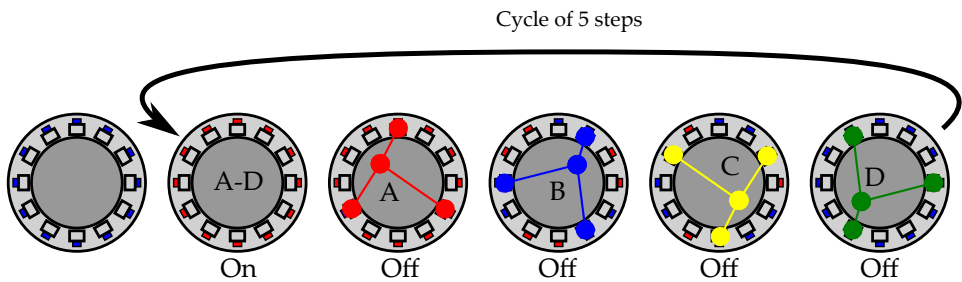
(c) Grouped in 3 section and 4 groups (A to D): n_f = 12 , n_s = 3 and n_g = 4 .
