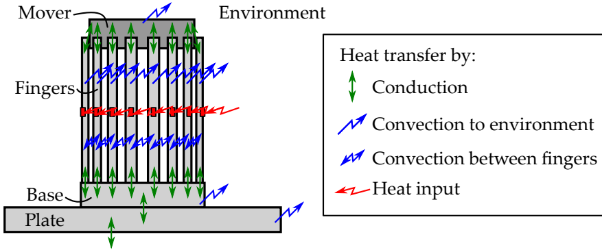
Figure B.1.: Thermal model definitions and heat flows.
