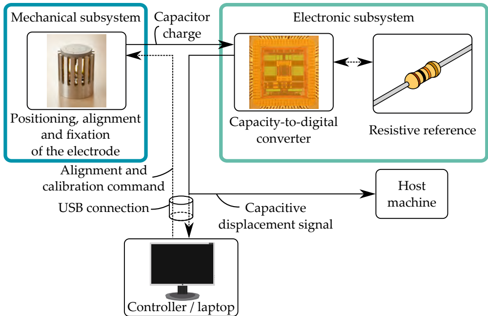
Figure 2.9.: System overview of the capacitive displacement measurement system. This picture is adapted from [Ven et al., 2012b]. The solid arrows indicate continuous communication whereas the dashed arrows indicate occasional or intermittent communication.
