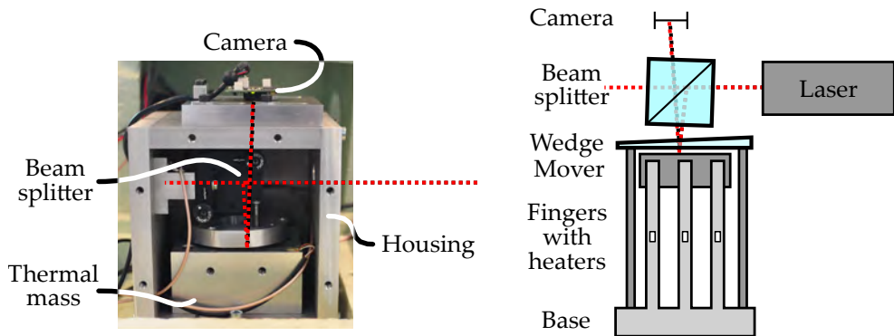
Figure C.1.: The Fizeau interferometer setup. (Setup by Jeroen van Schieveen.) The TSA is mounted within the thermal mass and is of the 16-finger type shown in Figure 4.5. The camera captures the interference pattern of the laser light (shown in Figure C.2a) reflected from the mover top-surface and the wedge bottom-surface. The spatial frequency and phase of the interference pattern are determined by the relative displacement and the tilt angles of the mover with respect to the wedge.
