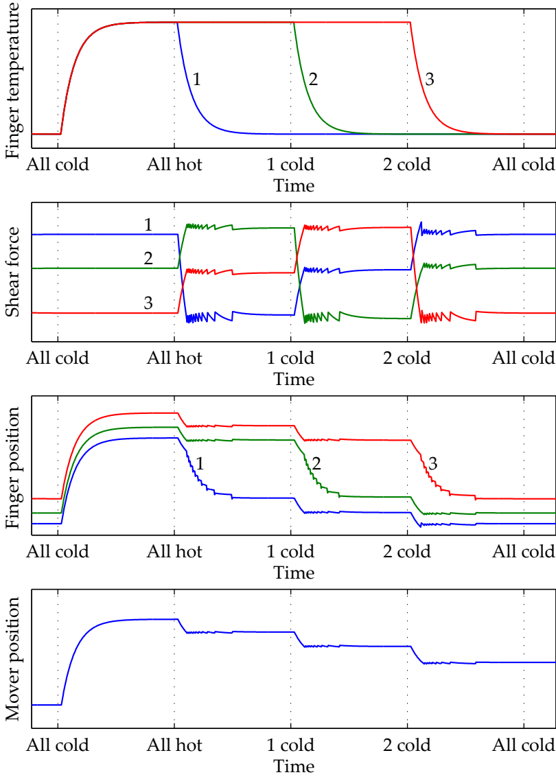
Figure 4.7.: Simulated temperatures and displacements of a simplified 3 finger TSA model. Whereas the simulation shown in Figure 4.3 only uses a static friction coefficient, in this simulation the friction is modelled using a static and a (30 % lower) dynamic friction coefficient. Also a shear-force graph is added to show the variations in the internal forces. The different lines in the three top graphs (shown in a different colour and with a different number) indicate the different fingers of the TSA. Stick-slip steps are clearly visible in this simulation. They were however never observed in practice, which in turn triggered the research described in Chapter 5. The model that is used is described in more detail in Appendix B.
