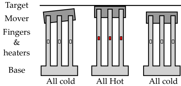
Figure 4.24.: Illustration of auto-alignment using the TSA. The mover is pushed to the target by heating all fingers and by applying thermal cycles. This aligns the surfaces to each other. The required mover-target distance is obtained by cooling down all fingers.
