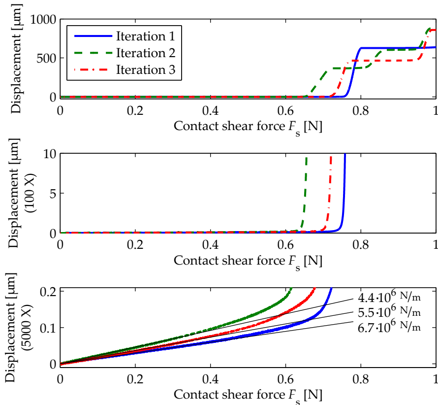
Figure 5.6.: Micrometre scale displacement response of a clean steel-steel friction contact to a contact shear force ( F_s ) increase from 0 to 1 N in 2 seconds. The experiment is repeated three times to show the effect of contact history. The variation in shear pre-load between the experiments is smaller than 10 mN and the contact normal force ( F_N ) equals 1.7 N. The stiffness of the contact (the initial slopes indicated in the bottom graph) and the force at which the first full sliding occurs varies significantly depending on the contact history.
