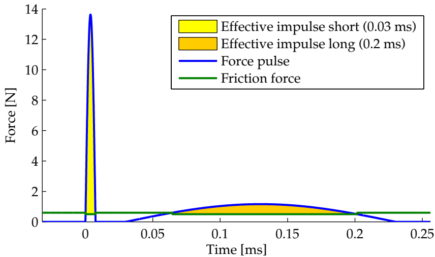
Figure 5.17.: Illustration of the interaction between a force pulse and the friction force for a short and a long pulse width. This graph shows that, when motion occurs if the force pulse magnitude is sufficient, and when the pulse displacement is determined by the impulse (the coloured areas in this graph), a large force and a small pulse width is recommended. The reason is that friction- and pulse-force variations have a relatively small impact on the impulse of the short pulse and thus on the displacement. The net impulse (the coloured area) of both force pulses is equal. Note that for this graph a simple static-kinetic friction coefficient was assumed. The real friction force variation during the pulse might be different. This graph is inspired on [Furst et al., 2010, Siebenhaar, 2004].
