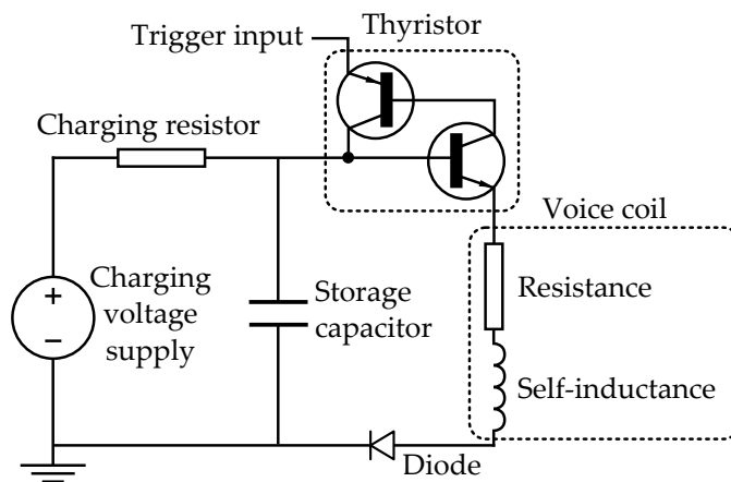
Figure 5.14.: Simplified schematic of the current pulse generating circuit. Energy is stored on the capacitor, which is in turn charged by the voltage supply. The charging resistor limits the charging current. When the thyristor is triggered, it closes the circuit so that current flows from the capacitor through the voice coil, generating an electromagnetic force in the voice coil. The thyristor opens when the current goes through zero, assisted by the diode.
