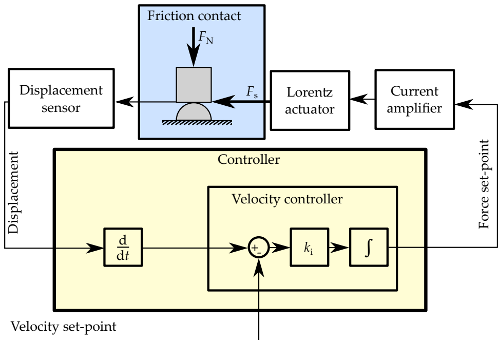
Figure 5.8.: Velocity controller structure. The yellow block represents the controller, the blue block the friction contact.
