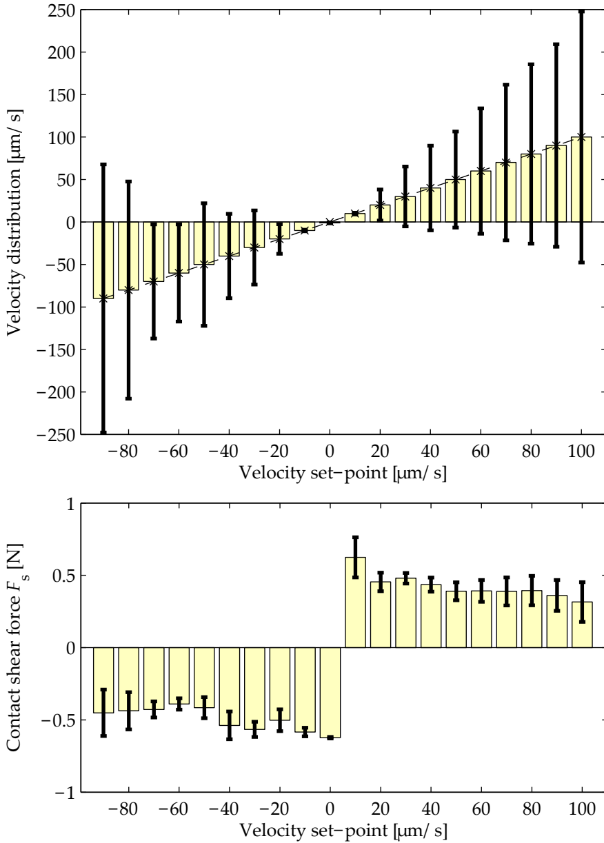
Figure 5.12.: Velocity control over a \pm 100 \mu\text{m/s} velocity range. The mean and standard deviation of the velocity and the contact shear force are shown for different velocity set-points. The dashed line/crosses in the top, velocity graph indicate the velocity set-points. For velocities of 20 \mu\text{m/s} and larger the velocity and force variations increase significantly as the unstable sliding regime is approached. Also, in contrast to the lower velocity behaviour shown in Figure 5.11, the shear force decreases for increasing velocities.
