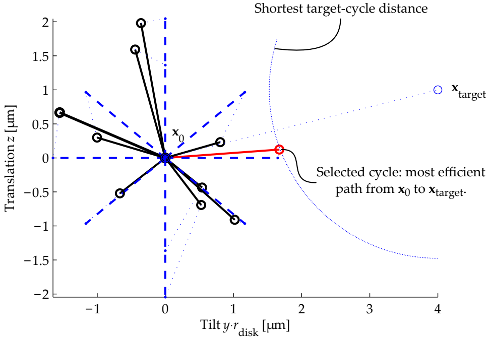
Figure 4.25.: Illustration of the cycle selection procedure for positioning with the TSA. For illustrative purposes the situation is simplified to 2 degrees of freedom: tilt around y and translation along z . The dashed lines represent ideal, estimated displacement steps, the solid lines represent the measured actuator motions. The dotted lines connect the measurement with the corresponding ideal motion. Note that the tilt axis is scaled with the electrode radius ( r_{\text{disk}} ) of 11 mm in order to have the same units on all axes. The positioning goal is to displace the mover from the current location \mathbf{x}_0 to \mathbf{x}_{\text{target}} . This is achieved by repeatedly selecting the cycle that results in the smallest position error. This is represented by the smallest circle around \mathbf{x}_{\text{target}} that touches an estimated actuator motion. This actuator motion (indicated in red) is selected and executed. The procedure is then repeated.
