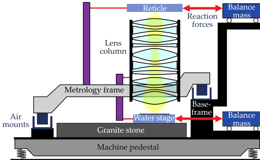
Figure 1.4.: Schematic representation of the architecture of a wafer scanner lithography system. This picture is adapted from [Munnig Schmidt et al., 2014].
