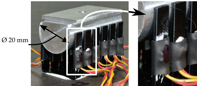
Figure 4.13.: Simplified thermal slider design using a standard heat-sink (an Aavid Thermalloy 504222B00000G). This aluminium heat-sink was selected such that the thermal crosstalk between the different fingers is small. The heating resistors are applied to the finger body using thermally conductive paste and heat-shrinkable tube. The heaters are controlled using an Arduino micro-controller board and a 16 channel LED driver.
