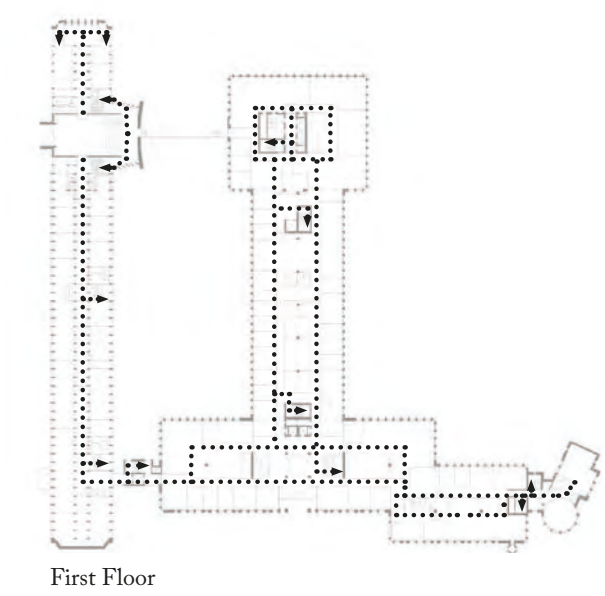
Circulation plans
