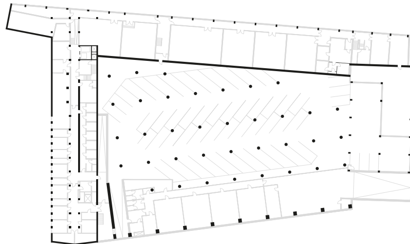
Basement
