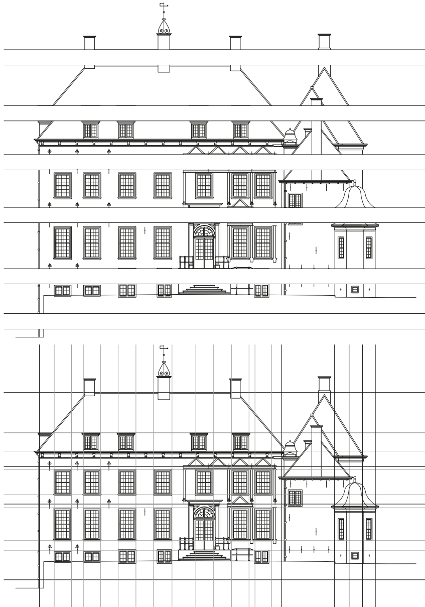
South façade main building
