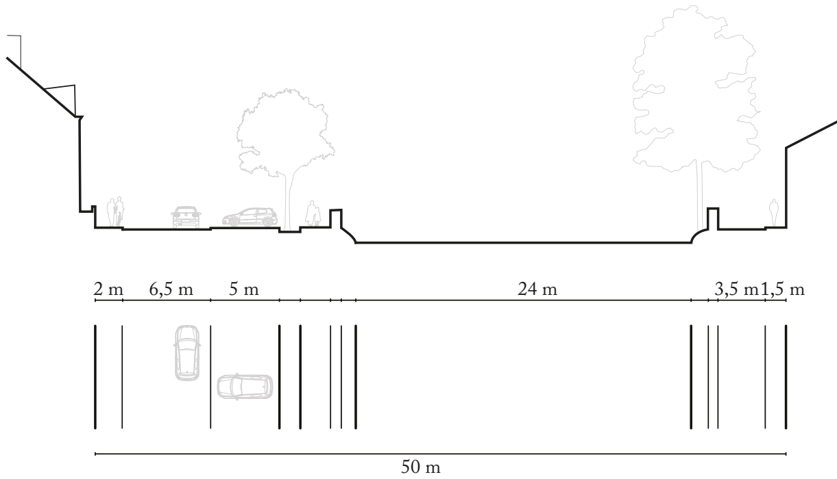
Section A
