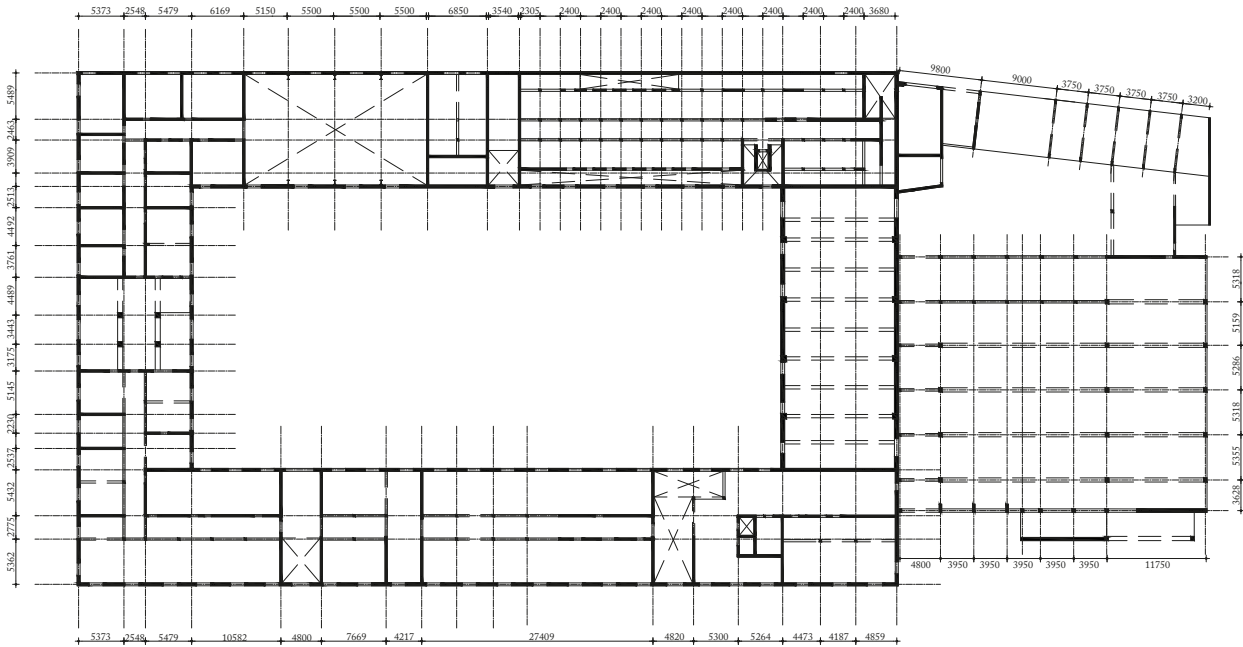
Structural grid
