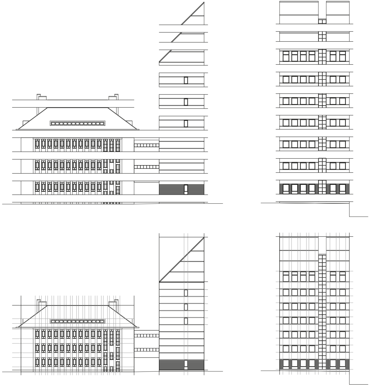
West façade
