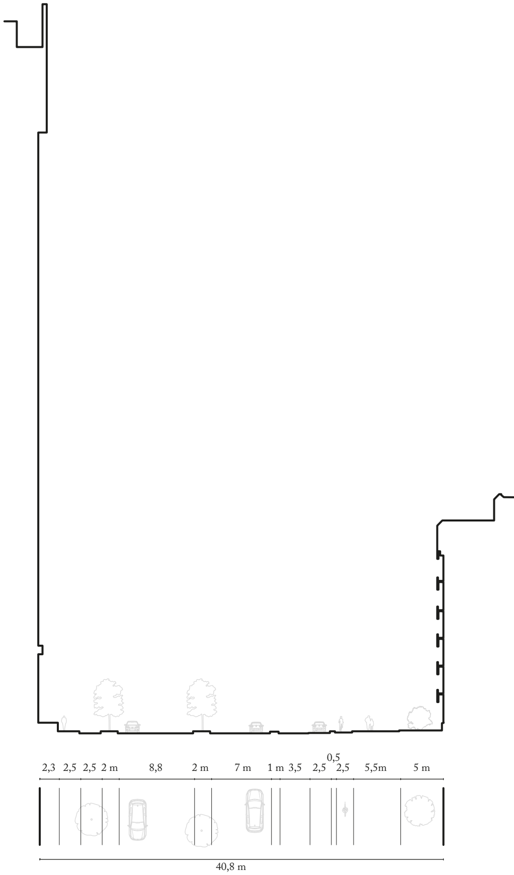
Section A
