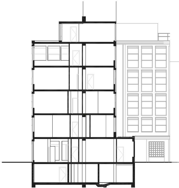
Section B
