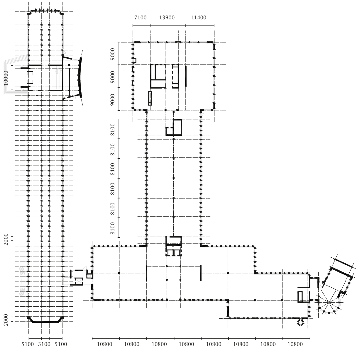
Structural grid
