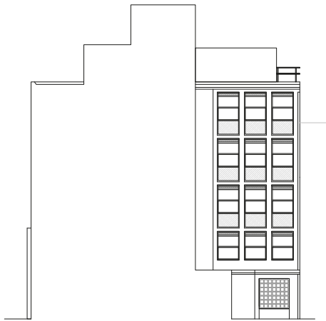
North façade
