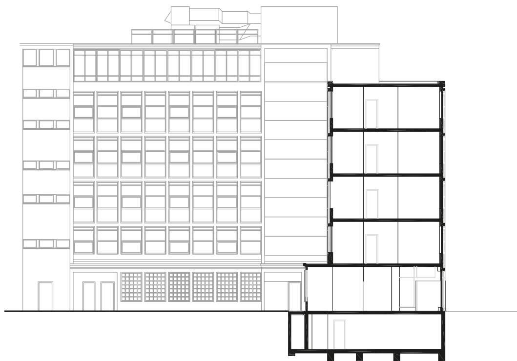
Section C
