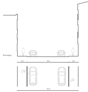
Section B
