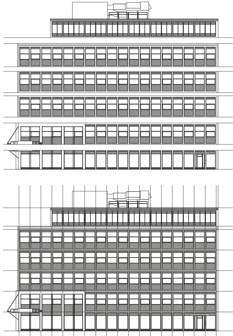
East façade
