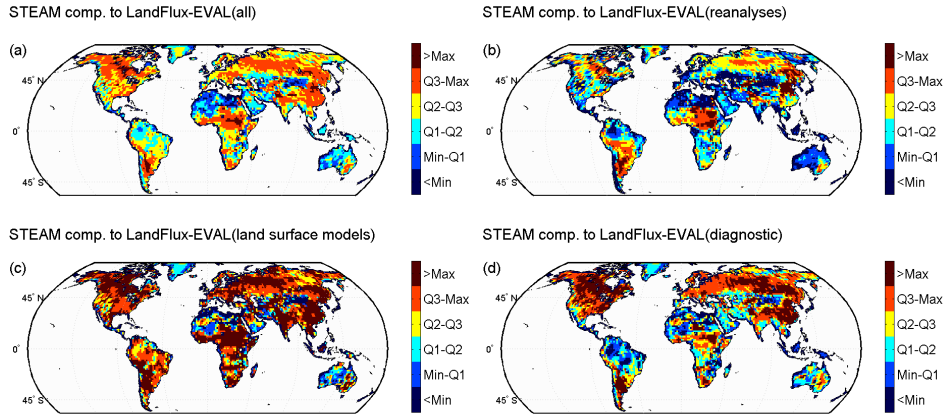
Figure 3.2: Annual mean STEAM evaporation compared to the statistics (minimum, first quartile, median, third quartile, maximum) of the LandFlux-EVAL product (1989–2005) for (a) merged synthesis, (b) reanalyses, (c) land-surface models, and (d) diagnostic data sets. Results are discussed in Sect. 3.4.1.
