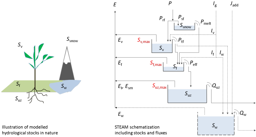
Figure 2.1: Water fluxes and stocks in STEAM. Arrows indicate fluxes, and boxes indicate stocks. Dashed lines indicate fluxes and stocks that only exist for particular land-use types. Symbols are listed in Notations.
