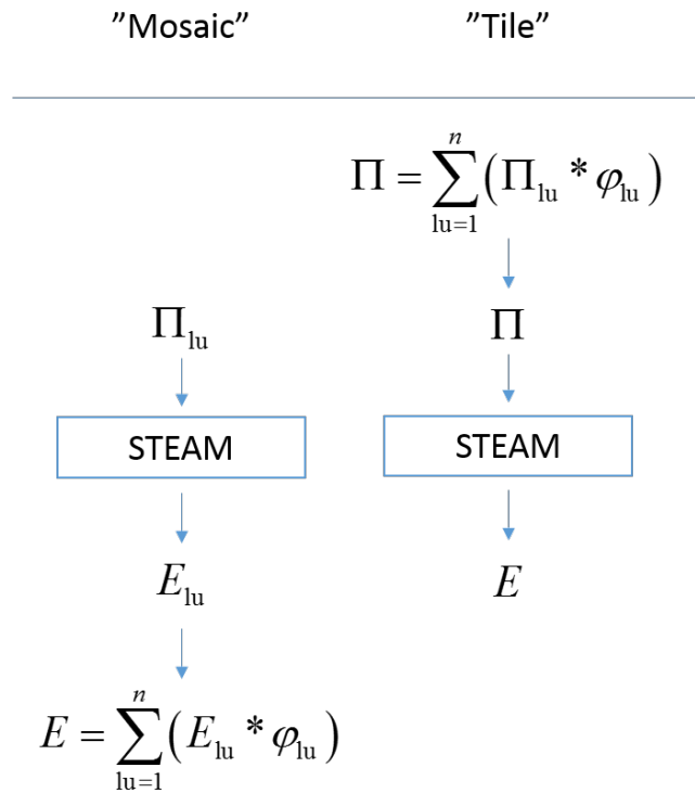
Figure 2.3: Parametrisation procedures in STEAM based on the 'mosaic' and 'tile' approach respectively.
