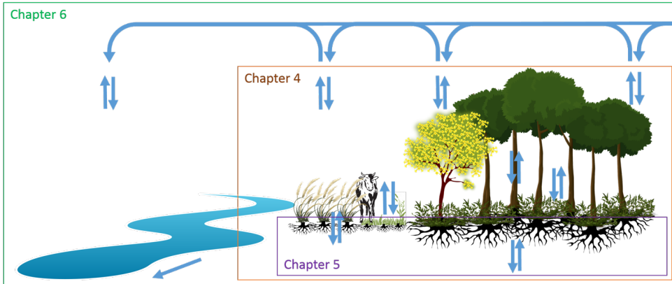
Figure 1.1: Different domains in the terrestrial water cycle covered by the different chapters. Chapter 4 focuses on the evaporation fluxes on land, Chapter 5 zooms in to the root zone storage capacity, and Chapter 6 zooms out to include moisture recycling and river flows.
