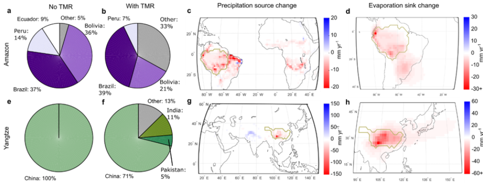
Figure 6.6: Nation influence of river flow change depending on consideration of terrestrial moisture recycling (TMR) in a-b , Amazon and e-f , Yangtze. Without TMR, the nation influence on river flow change originates entirely from within-basin country-wise evaporation change ( a , e ). By considering TMR, the nation influence ( b , f ) is the sum of absolute imported precipitation change (precipitation source outside encircled basin boundaries in c and g ) and of absolute exported evaporation change (evaporation sink outside encircled basin boundaries in d and h ) (Sect. 6.2). Precipitation sources ( c , g ) and evaporation sinks ( d , h ) within basin boundaries are recycled.
