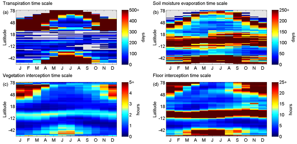
Figure 4.2: Changes in terrestrial timescales (Eq. 4.1) over the year and different latitudes (1999–2008). Note that the units are in hours for E_v and E_f , and in days for E_t and E_{sm} . Grey indicates when a timescale approaches infinity. Results are discussed in Sect. 4.3.1
