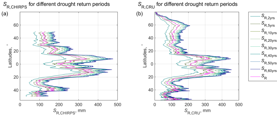
Figure 5.10: Mean latitudinal root zone storage capacity (a) S_{R,CHIRPS-CSM} (based on P_{CHIRPS} and E_{CSM} ) and (b) S_{R,CRU-SM} (based on P_{CRU} and E_{SM} ) dimensioned by drought return periods between 2 and 60 years estimated using Gumbel distribution (see methods described in Sect. 5.2.3).
