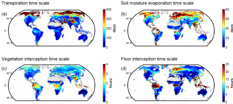
Figure 4.1: Average surface timescales of different evaporation fluxes: (a) transpiration, (b) soil moisture evaporation, (c) vegetation interception, and (d) floor interception (1999–2008). Grey indicates grid cells with mean evaporation rates below 0.01 \text{ mm d}^{-1} . Note that the units are in hours for E_v and E_f , and in days for E_t and E_{sm} ; see Eq. (4.1). Results are discussed in Sect. 4.3.1.
