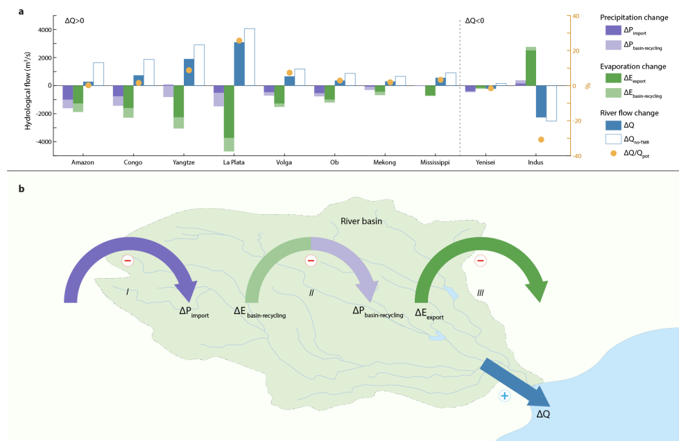
Figure 6.5: Changes in hydrological flows at river basin scale. a , Changes in hydrological flows by ten basins with the largest terrestrial moisture recycling (TMR) effect on river flows: eight basins with increased and two with decreased river flows ( Q ). Basins are ordered by maximum absolute TMR effect on river flows, i.e., the difference between river flows with or without TMR ( \Delta Q - \Delta Q_{\text{noTMR}} ). b , Conceptual figure of hydrological flow changes in a basin. The (-) and (+) as displayed here are e.g. seen in Amazon, Congo, Volga. In Indus and Yenisei, the (-) and (+) are reversed.
