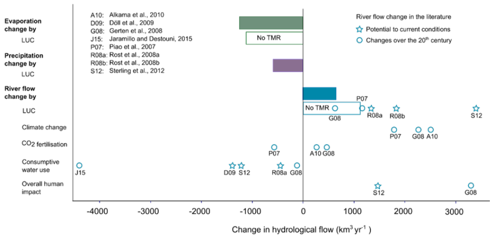
Figure 6.3: Human impact on global hydrological flows. The solid bars show our estimated net change (terrestrial area 131,710,600 \text{ km}^2 and time period 2000–2013) in evaporation, precipitation and river flows including consideration of terrestrial moisture recycling (TMR). Hollow bars show flow changes without TMR. Circles and stars indicate river flow change estimates from other studies, where land-use change (LUC) implicitly accounts for consumptive water use. Note that while consumptive water use alone always reduces river flows, other human impacts have both positive and negative influences that are concealed by the global aggregate.
