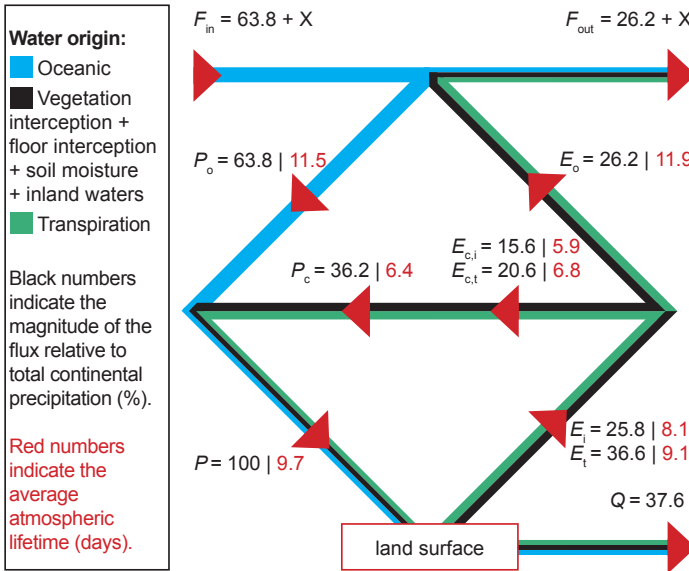
Figure 4.4: Global hydrological cycle over land, i.e., all continents considered together (1999–2008). F_{in} is the atmospheric moisture of oceanic origin that crosses the ocean-land boundary and enters the atmosphere above land. F_{out} is the atmospheric moisture that leaves the ocean-land boundary towards the ocean. Thus, X represents the atmospheric moisture of oceanic origin that passes through the continental atmosphere, but never precipitates. Precipitation on land P (set to 100%) is composed of moisture evaporated from the ocean P_o and a recycled part P_c . On the land surface water runs off Q , or evaporates through direct evaporation E_i or through transpiration E_t . Part of this evaporation is lost to the ocean E_o , while other parts of the evaporation recycle E_{c,i} and E_{c,t} . Evaporation data are from STEAM, precipitation data are from ERA-I, the recycled fractions and lifetimes are calculated by WAM-2layers (van der Ent et al., 2014) and the other terms follow from the water balance.
