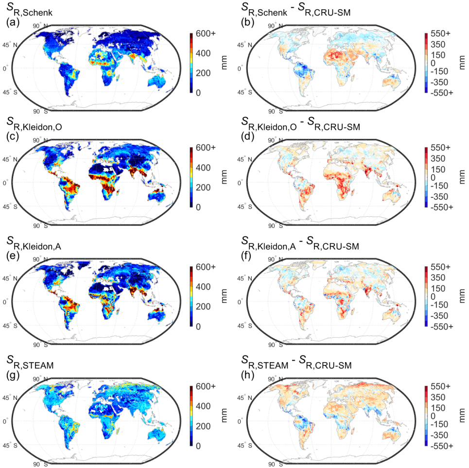
Figure 5.6: Root zone storage capacities of (a) S_{R,Schenk} (Schenk and Jackson, 2009), (c) S_{R,Kleidon,O} (Kleidon, 2004), (e) S_{R,Kleidon,A} (Kleidon, 2004), (g) S_{R,STEAM} (based on look-up table in Wang-Erlandsson et al. (2014)) and (b, d, f, h) their differences with S_{R,CRU-SM} (estimated based on E_{SM} and P_{CRU} in this study). Values below 0.5% of the maximum in (a), (c), (e), and (g) are displayed as white.
