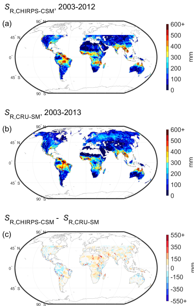
Figure 5.5: Root zone storage capacity estimates of (a) S_{R,CHIRPS-CSM} (based on P_{CHIRPS} and E_{CSM} ), (b) S_{R,CRU-SM} (based on P_{CRU} and E_{SM} ), and (c) the difference between S_{R,CHIRPS-CSM} and S_{R,CRU-SM} . Values below 0.5 % of the maximum in (a) and (b) are displayed as white.
