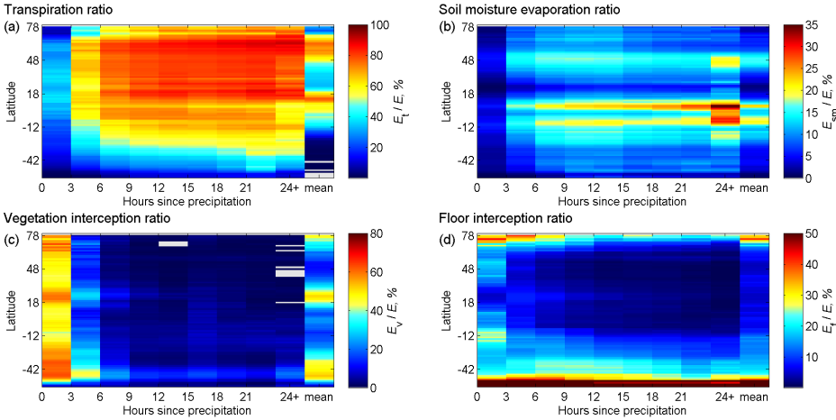
Figure 4.3: Evaporation partitioning with time since precipitation over terrestrial latitudes (1999–2008). Results are discussed in Sect. 4.3.2.
