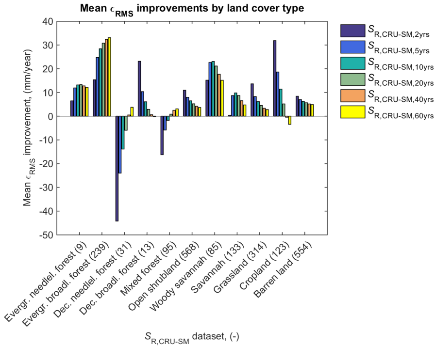
Figure 5.11: The mean \epsilon_{RMS} improvement in simulated monthly evaporation E (2003–2013) by implementing S_{R,CRU-SM,Lyrs} (based on P_{CRU} and E_{SM} ) instead of S_{R,STEAM} (based on look-up table in Wang-Erlandsson et al. (2014)) in the global hydrological model STEAM, where the satellite based E_{SM} was used as the benchmark for improvements (see methods described in Sect. 5.2.2). The improvements for root zone storage capacities with different return periods L 2–60 yrs (i.e., S_{R,CRU-SM,2yrs} , S_{R,CRU-SM,5yrs} , S_{R,CRU-SM,10yrs} , S_{R,CRU-SM,20yrs} , S_{R,CRU-SM,40yrs} , and S_{R,CRU-SM,60yrs} ) are shown for the different land-cover types that has >90 % grid cell coverage. The number of represented grid cells are provided in the parenthesis following each land-cover type label along the x-axis.
