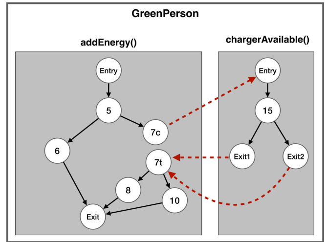
Fig. 4. CCFG of GreenPerson as subclass.
