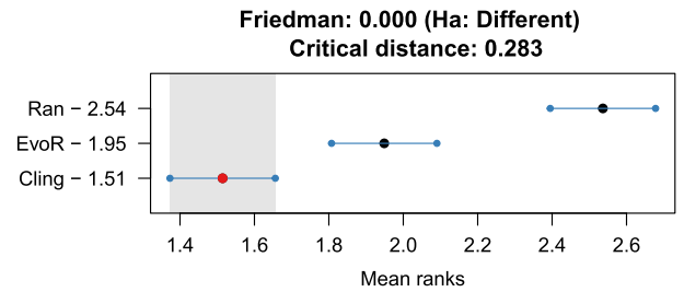
Fig. 7. Non-parametric multiple comparisons (i.e., mean ranks with confidence interval) in terms of CBC score for T_{\text{CLING}} (Cling), T_{\text{EvoR}} (EvoR), and T_{\text{Ran}} (Ran) using Friedman's test with Nemenyi's post-hoc procedure.
