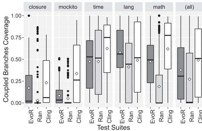
Fig. 6. Total coupled-branches coverage achieved by T_{\text{CLING}} (Cling), T_{\text{Ran}} (Ran) and T_{\text{EvoR}} (EvoR). ( \diamond ) denotes the arithmetic mean and (—) is the median.
