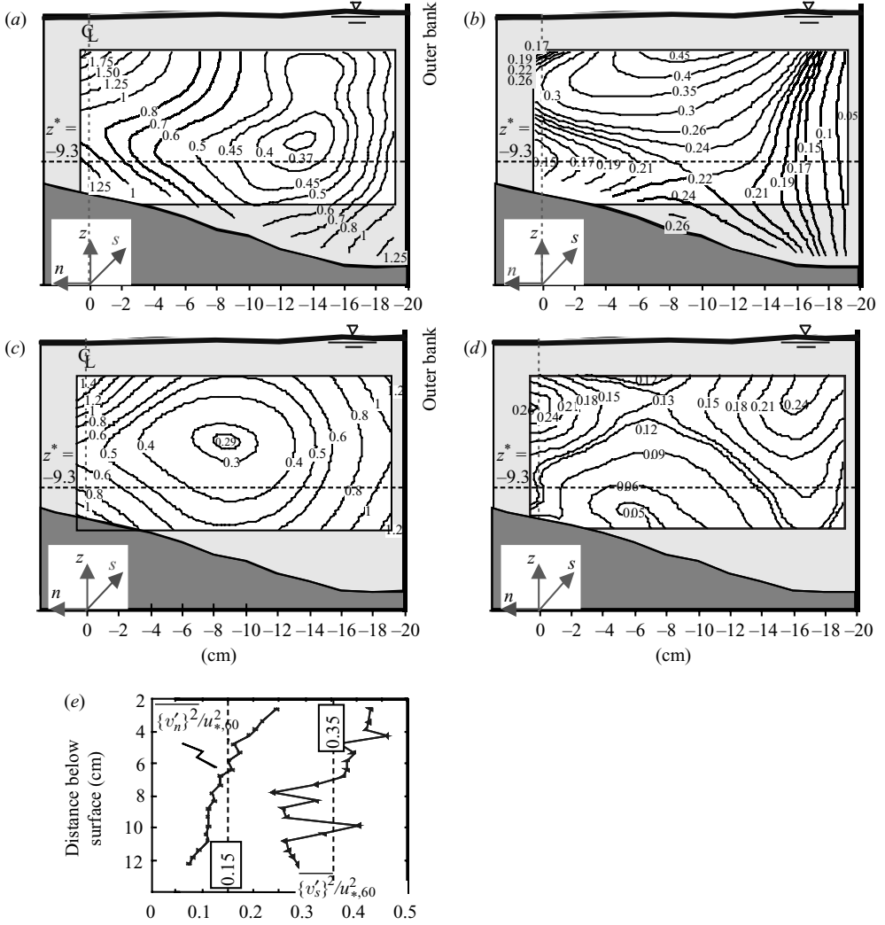
FIGURE 9. Turbulent normal stresses (a) \overline{v'^2} and (b) \overline{v_n'^2} ; contributions to normal stresses by background turbulence (c) \overline{v_{s,b}'^2} and (d) \overline{v_{n,b}'^2} ; and (e) by width-coherent fluctuations \{\overline{v_s'^2} and \{\overline{v_n'^2} . All normalized by u_{*,60}^2 .
