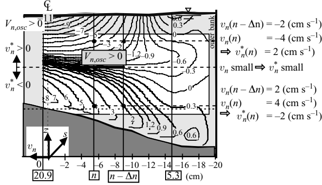
FIGURE 7. Isolines of transversal velocity, v_n (cm s -1 ), to illustrate how a bulk transversal displacement \Delta n of the entire pattern leads to variations of the Eulerian transversal velocity.
