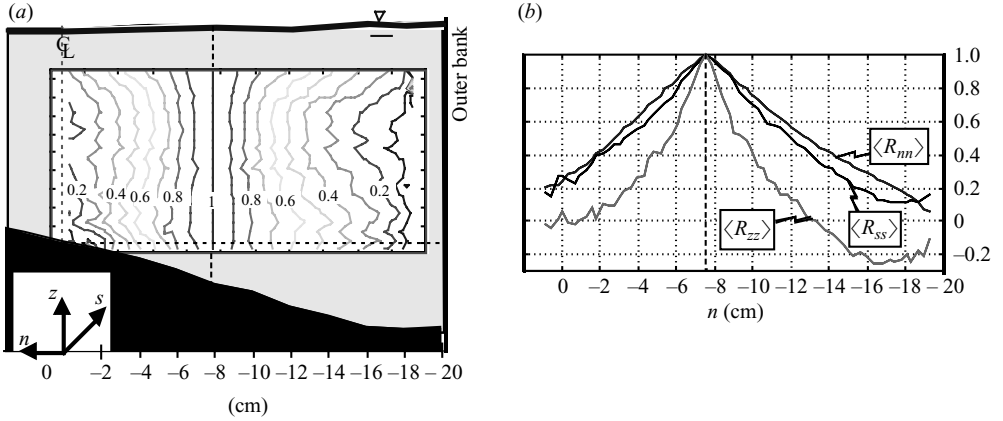
FIGURE 6. (a) Two-point correlation R_{nn}(-7.5, n; z) between the transversal velocity fluctuations measured at 12.5 cm from the outer bank and points on the same transversal profile; (b) Vertically-averaged two-point correlations, \langle R_{jj} \rangle (j = s, n, z) .
