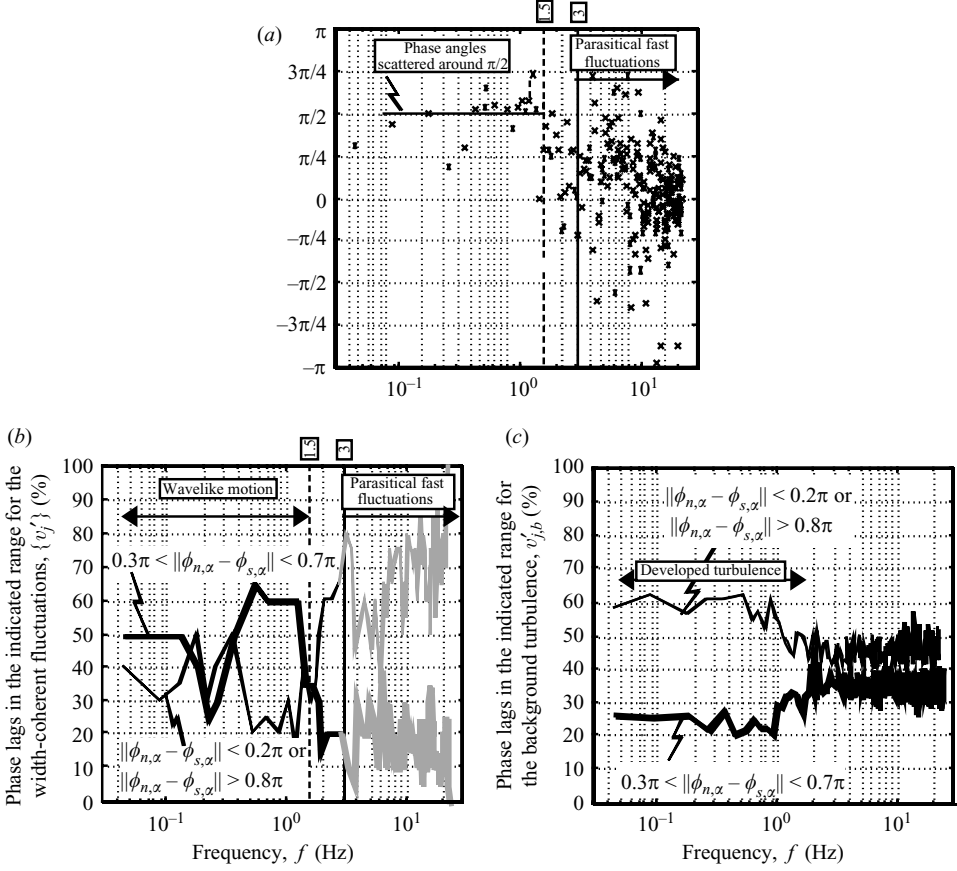
FIGURE 12. Phase lags \phi_{n,\alpha} - \phi_{s,\alpha} between (a) width-coherent fluctuations \{v'_f\} and \{v'_n\} for profile at 9.3 cm below water surface; (b) width-coherent fluctuations \{v'_f\} and \{v'_n\} averaged over measuring grid; (c) background-turbulence fluctuations v'_{s,b} and v'_{n,b} averaged over measuring grid.
