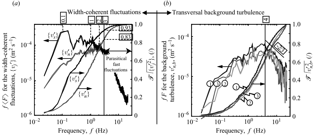
FIGURE 11. (a) Frequency \times power spectral density, f\langle F \rangle , and normalized cumulative power spectral density, \mathfrak{I}/\langle v'_j \rangle^2 , for width-coherent fluctuations, \{v'_s\} and \{v'_n\} , averaged over all measured profiles; (b) frequency \times power spectral density, fF and normalized power spectral density, \mathfrak{I}/v'^2_{n,b} , for transversal background turbulence, v'_{n,b} , in three points with coordinates (1) (n, z^*) = (-12, -9.3) ; (2) (-7.5, -9.3) ; (3) (-3, -9.3) .
