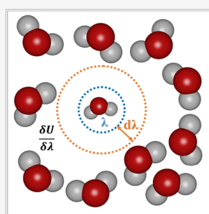
Thermodynamic Integration
