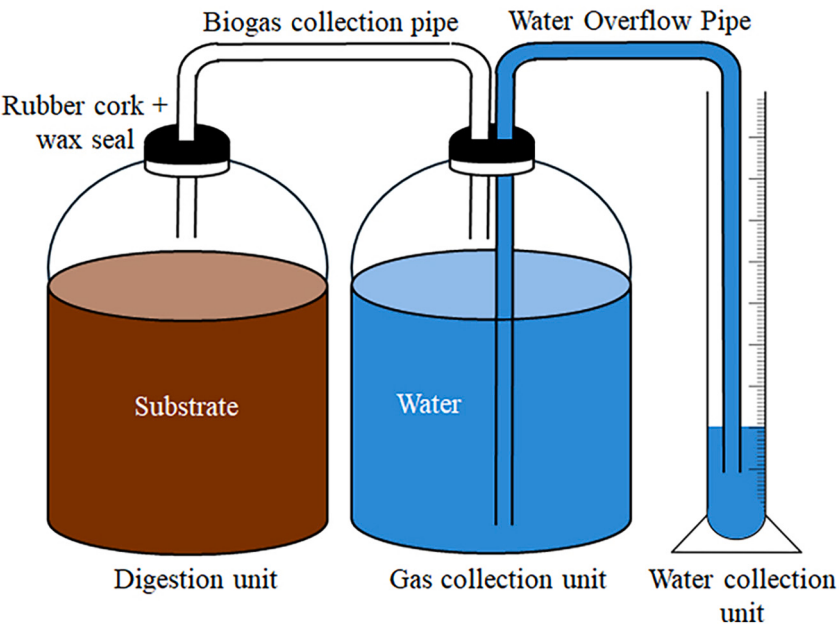
Fig. 1. Biogas production reactor diagram.
