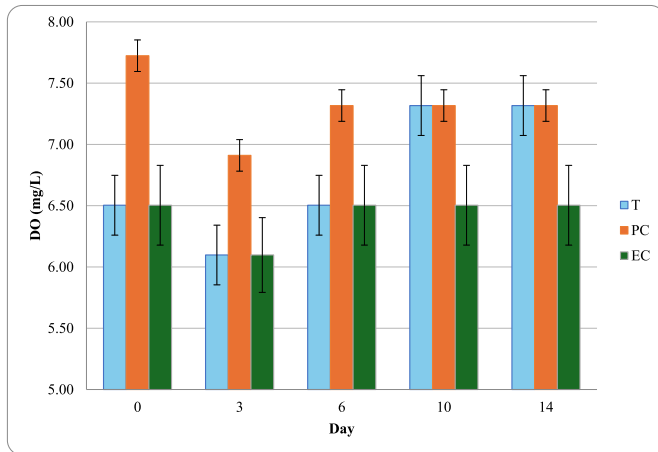
Fig. 6. DO concentration during phytotreatment (T: treatment, PC: plant control, and EC: effluent control).
