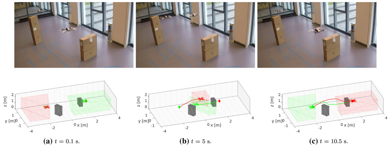
Fig. 11 Collision avoidance with two quadrotors and two static obstacles. The two quadrotors are required to swap their positions. Top row: Snapshots of the experiment. Bottom row: Trajectories of the robots.
