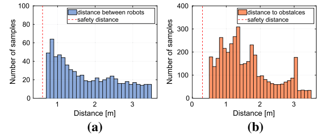
Fig. 10 Experimental results with two differential-drive robots. a Histogram of inter-robot distance. b Histogram of distance between robots and obstacles
