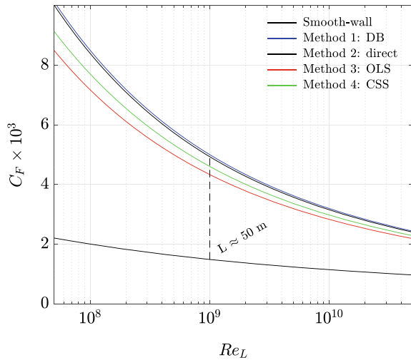
Fig. 3 Prediction of the averaged frictional drag C_F as a function of fetch Reynolds number Re_L at a unit Reynolds number U_\infty/\nu \approx 2 \times 10^7 with U_\infty \approx 18 \text{ ms}^{-1} and \nu \approx 9 \times 10^{-7} \text{ m}^2 \text{ s}^{-1}
