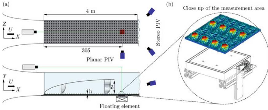
Fig. 1 a Schematics of the experimental setup of the planar and stereo-PIV and b a close-up of the floating-element drag balance with the surface topography of a single repeating unit
