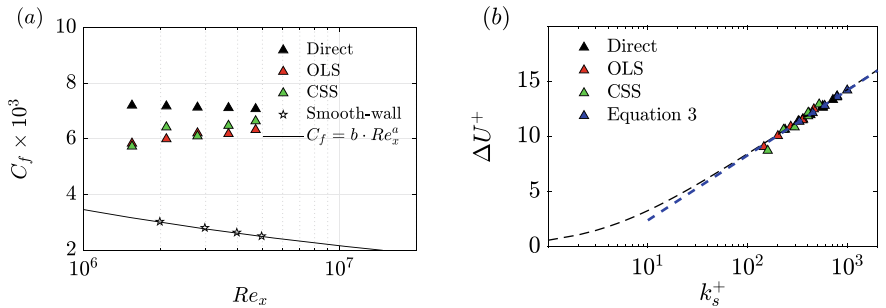
Fig. 2 a Variation of the skin-friction coefficient estimated using different methods for Config 1, with the smooth-wall data from [5], and the black solid line representing Schlichting's power-law. b Variation of the roughness function estimated the direct and indirect methods, with the solid black line representing the fully rough asymptote
