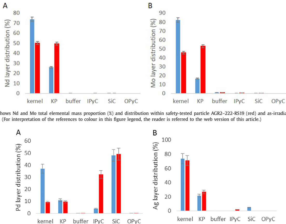
Fig. 11. (a, b). Shows Pd and Ag total elemental mass proportion (%) and distribution within safety-tested particle AGR2-222-RS19 (red) and as-irradiated particle AGR2-223-RS34 (blue). (For interpretation of the references to colour in this figure legend, the reader is referred to the web version of this article.)
