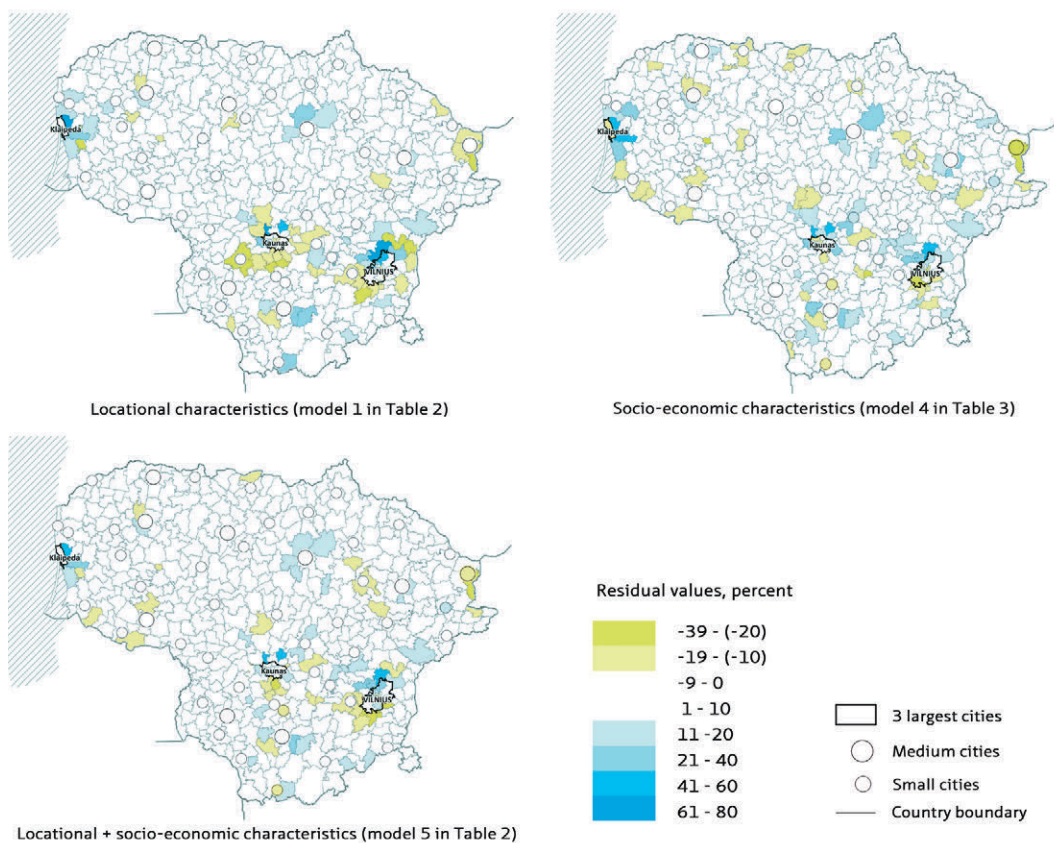
FIGURE 2.5 Residuals of various models
