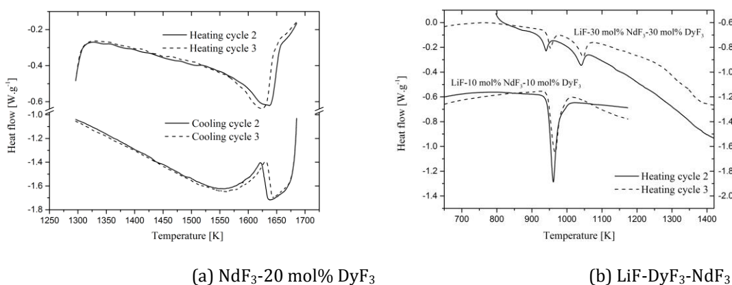
Figure 6.1– DTA thermograms of representative compositions.
