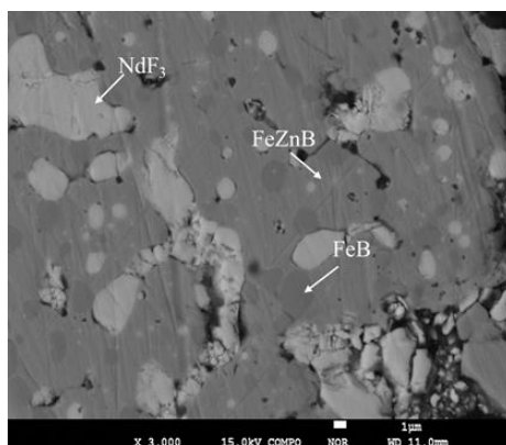
Figure 3.7- BSE image of the LiF-NdFeB-ZnF 2 sample in at% after fluorination treatment showing the presence of NdF 3 , FeB and FeZnB.
