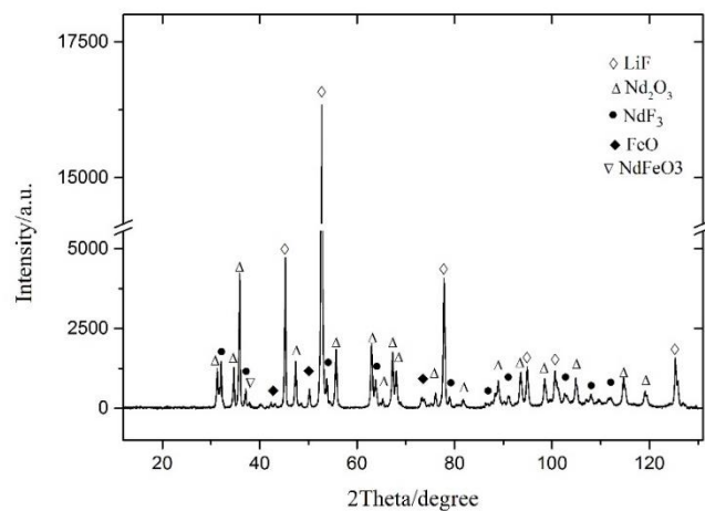
Figure 5.15– XRD result of the sample of LiF-Nd 2 O 3 -FeF 3 electrolyte after electrolysis with iron anode and Mo cathode.
