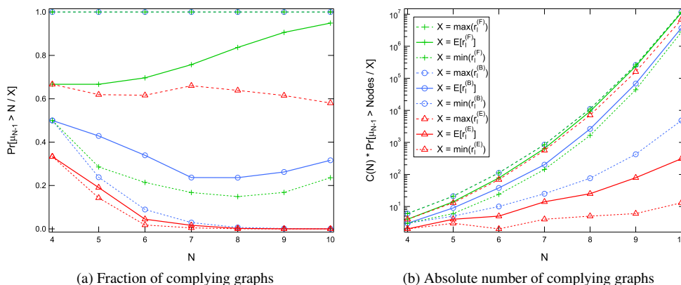
FIG. 3: Number of graphs that obey the indicated inequalities for networks sizes in the range [4, 10] , both as a percentage and as an absolute number (left image and right image, respectively). The top dashed curve represents C(N) , i.e. the total number of non-isomorphic connected graphs with N nodes. The legend applies to both images.
