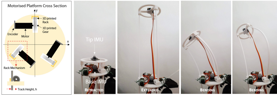
Fig. 2. Design of the actuation stages of the manipulator showing the triaxial motors and 3D printed tracks. Accompanied by pictures showing the range of motions and actions that can be achieved using the manipulator. The placement of the IMUs is highlighted.
