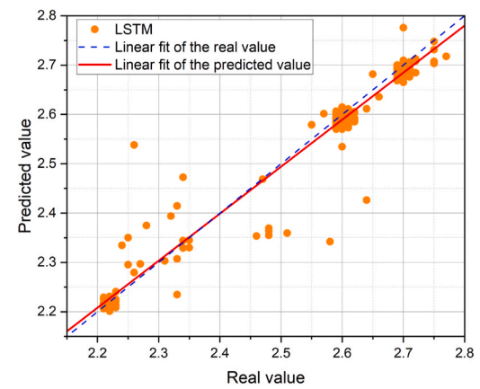
d) LSTM
