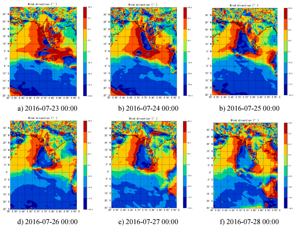
Fig. 4. The spatiotemporal distribution characteristics of wind directions.
