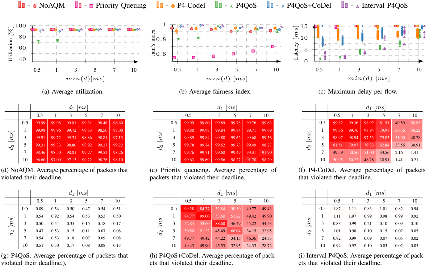
Fig. 3: Evaluation using the Tofino switch (topology 2a). Confidence intervals 95%.
