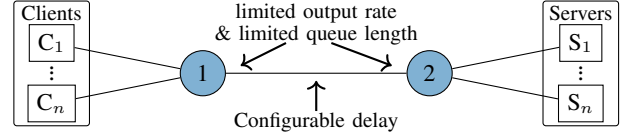
(a) Single bottleneck topology (2-switches, 1 links).
