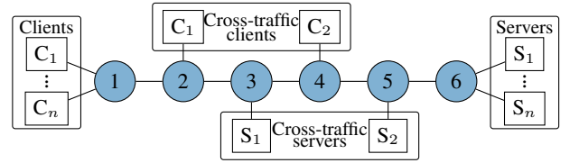
(b) Multiple-bottlenecks topology (6-switches, 5 links).
