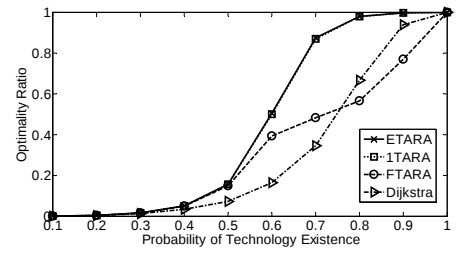
(b) Lattice
