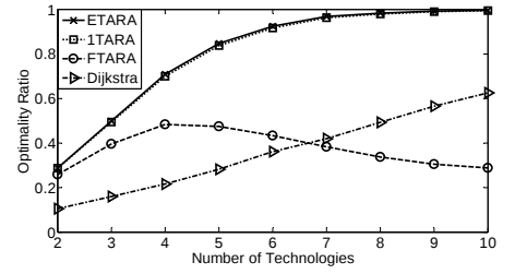
(b) Lattice
