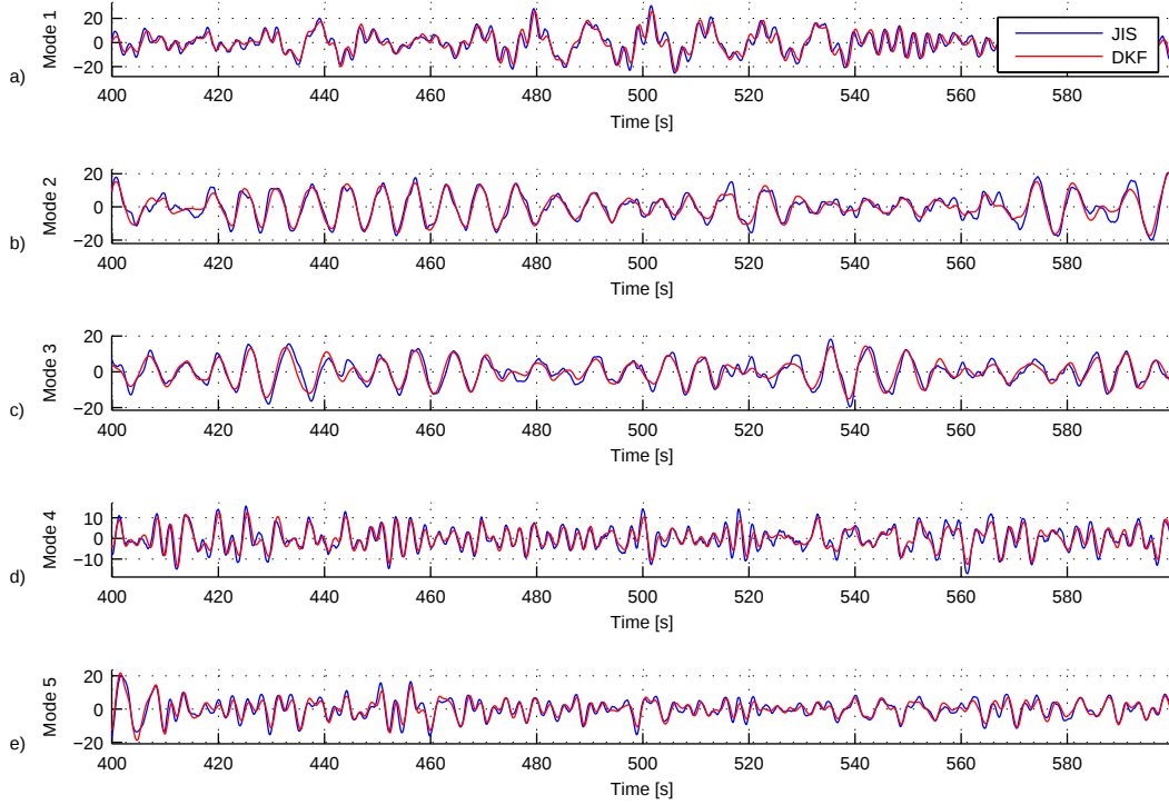
Figure 8: Estimation of the five lowermost modes in the model
