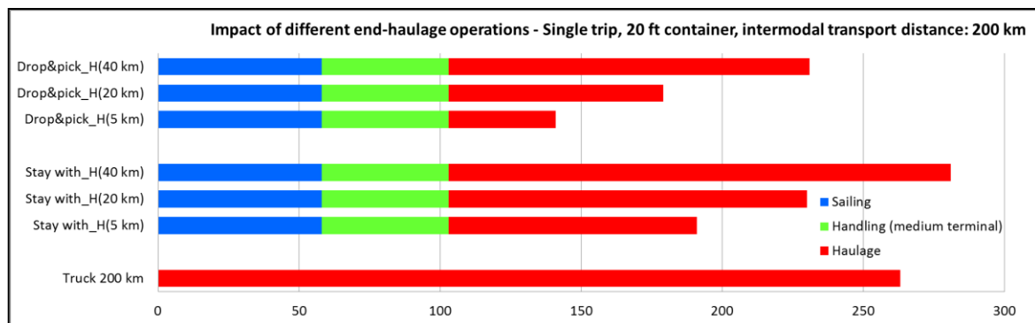
Figure 10 Impact of different end-haulage operations on cost competitiveness of intermodal IWT (at 200 km)
