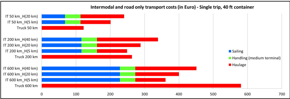
Figure 6 Impact of load unit size on cost competitiveness of intermodal IWT
