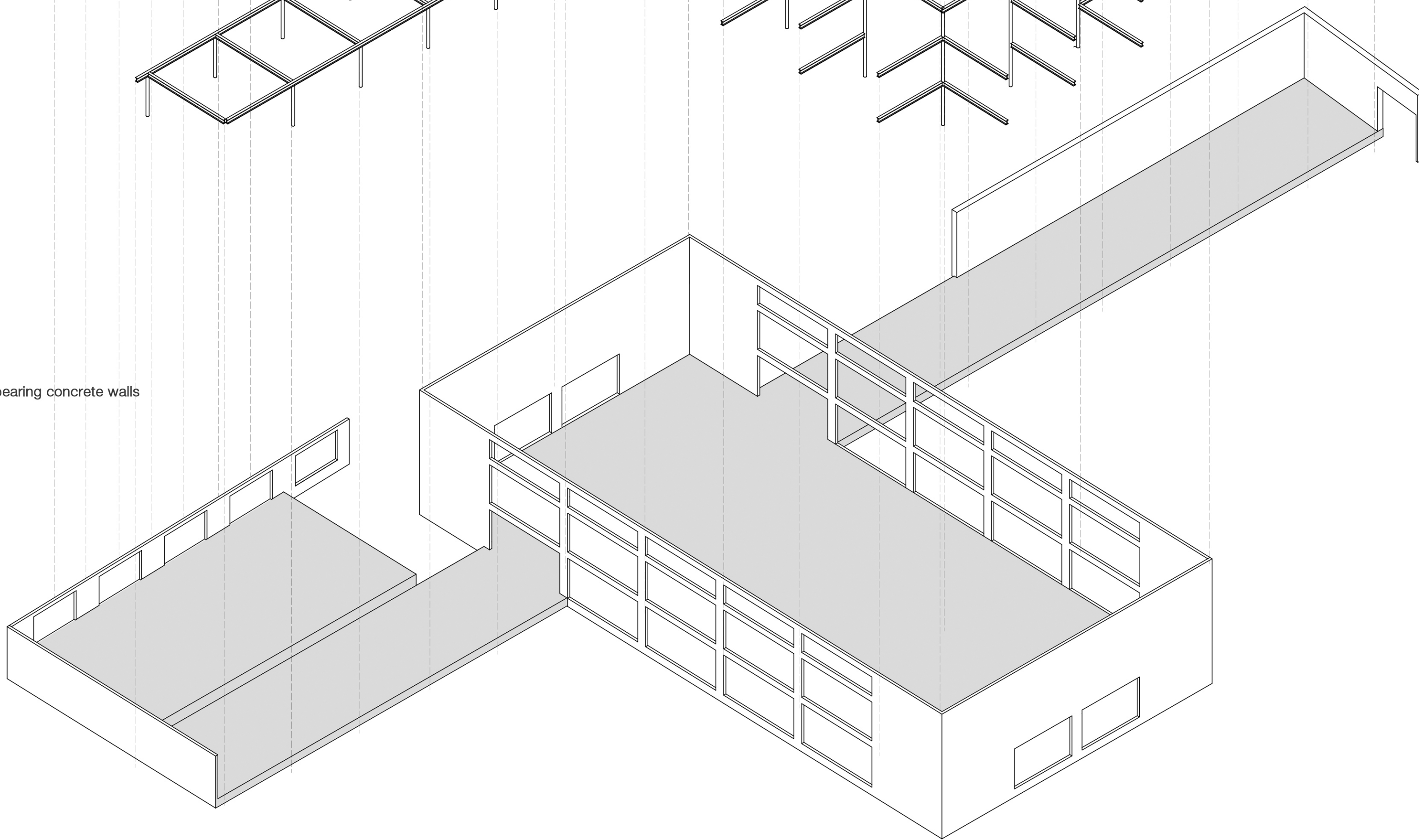
Load-bearing Structure
