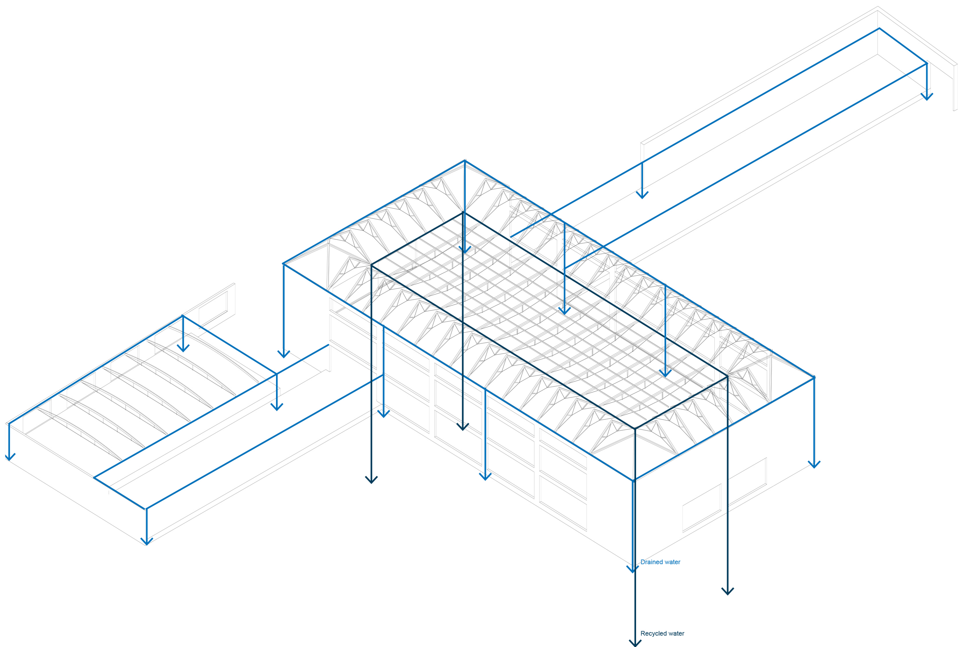
Rainwater drainage
