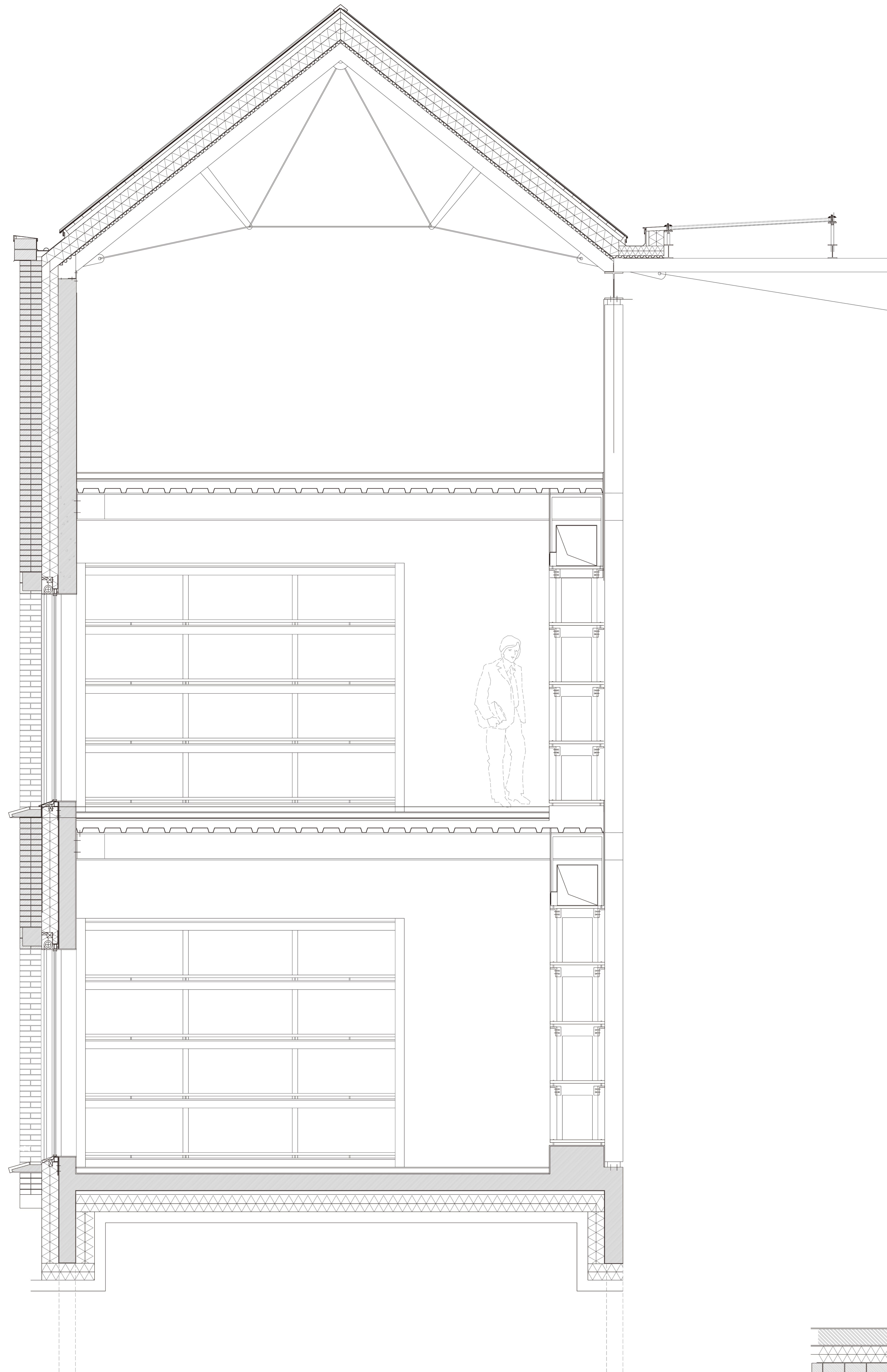
Detail Section 1: 20
