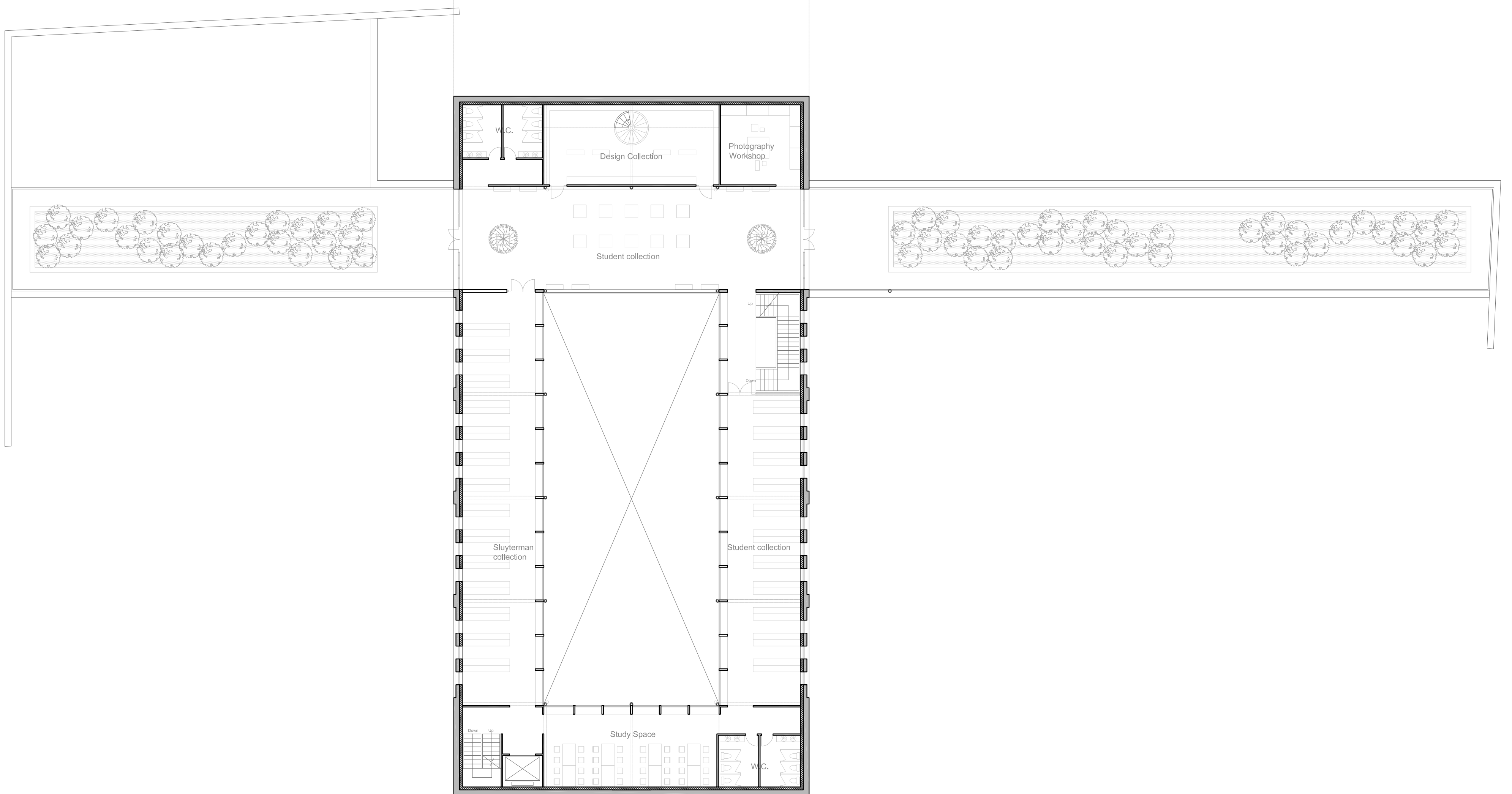
First Floor Plan 1:200
