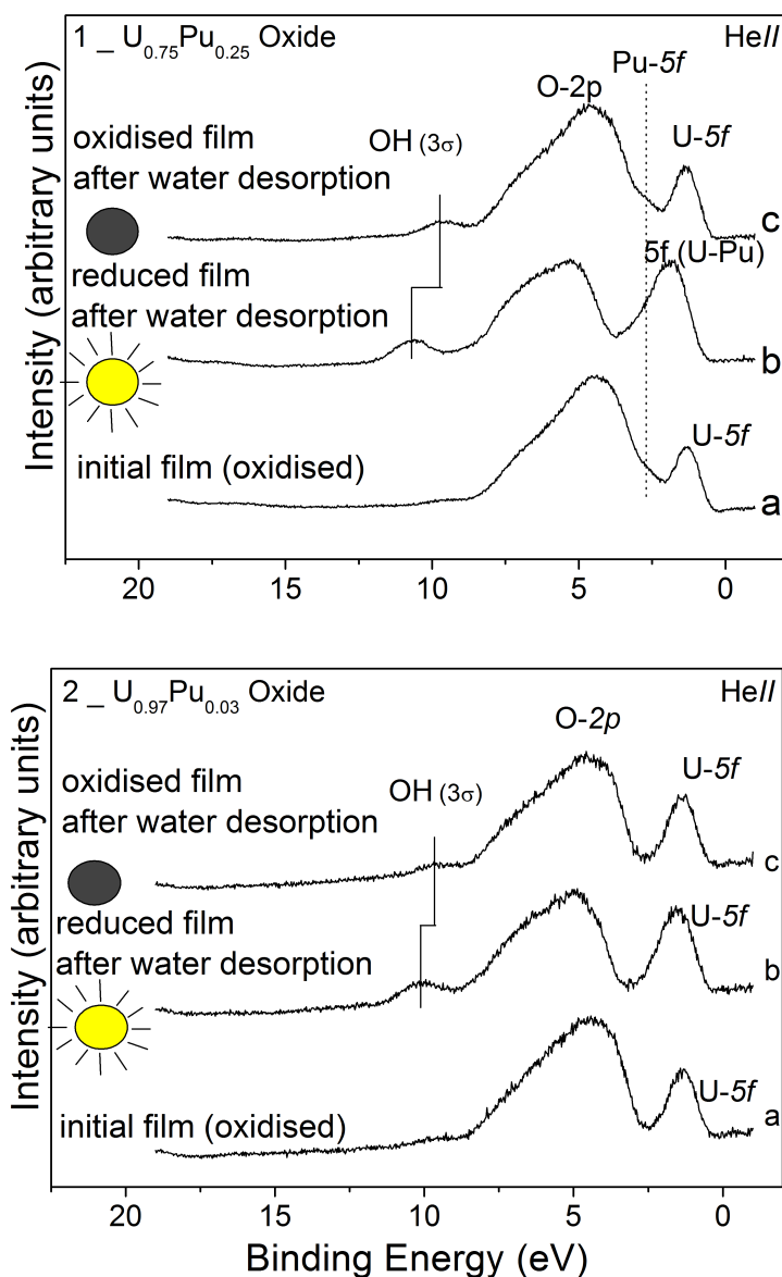
Figure 5.6: HeII valence band spectra comparison of irradiated and dark areas of (1) \text{U}_{0.75}\text{Pu}_{0.25} oxide and (2) \text{U}_{0.97}\text{Pu}_{0.03} oxide thin films after ice desorption.
