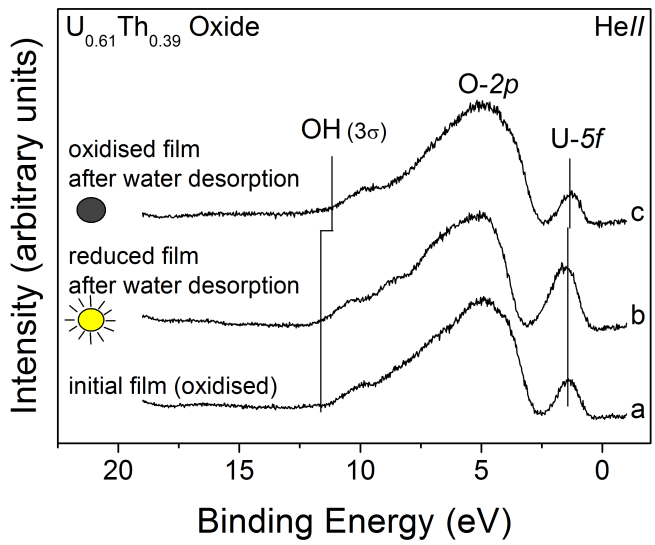
Figure 5.9: HeII valence band comparison of irradiated and dark areas of \text{U}_{0.61}\text{Th}_{0.39}\text{ oxide} .
