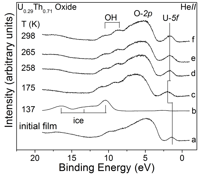
Figure 5.8: HeII valence band spectra of \text{U}_{0.29}\text{Th}_{0.71}\text{ oxide} after ice adsorption and desorption under UV light.
