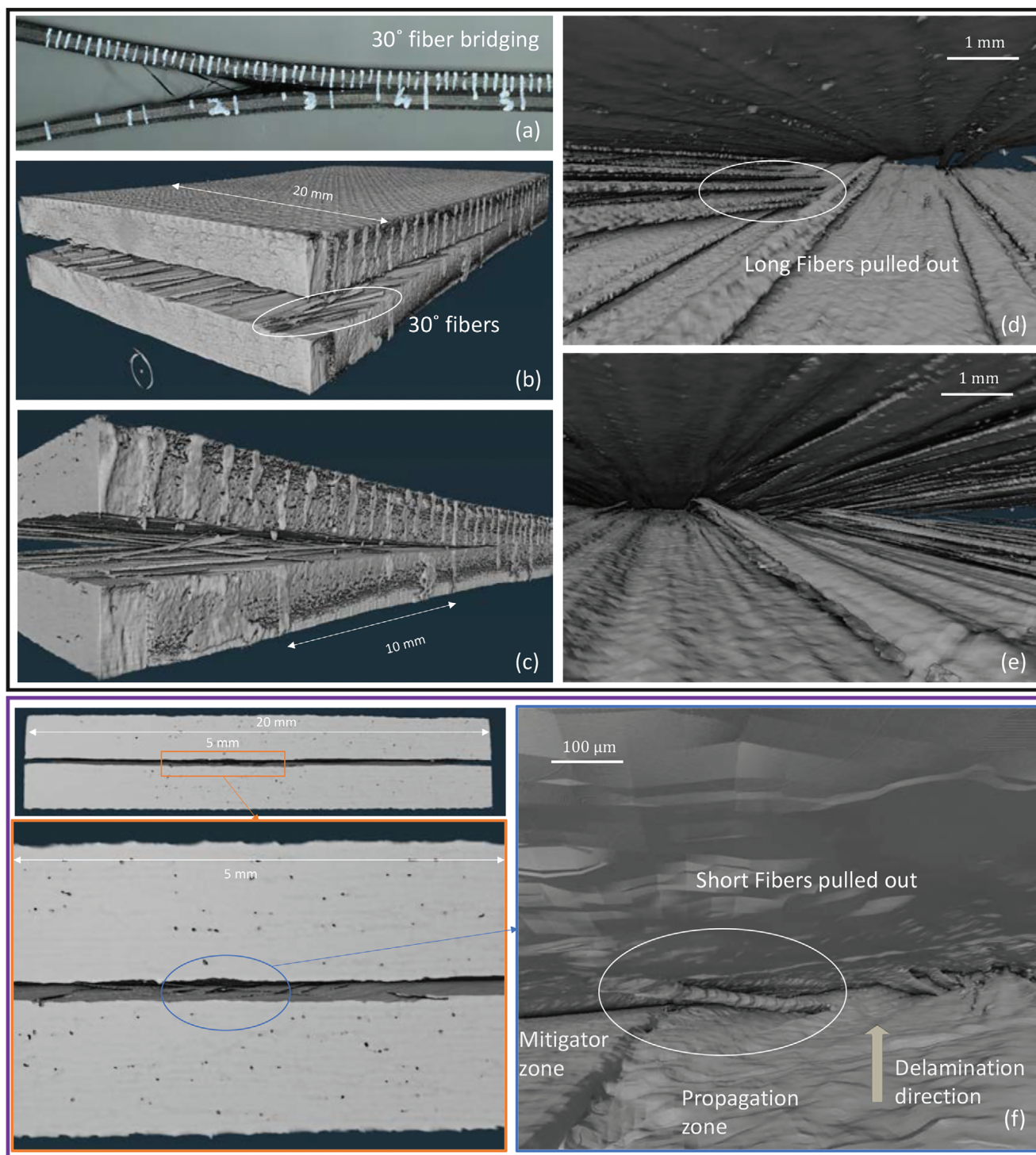
Figure 7. Delamination of multidirectional FRP (30°/30°) showing: a–e) Fully developed LSB in delamination width of 20 mm, and f) Short fiber bridging in delamination width of 5 mm. Reproduced with permission. [101] Copyright 2022, Elsevier B.V.
