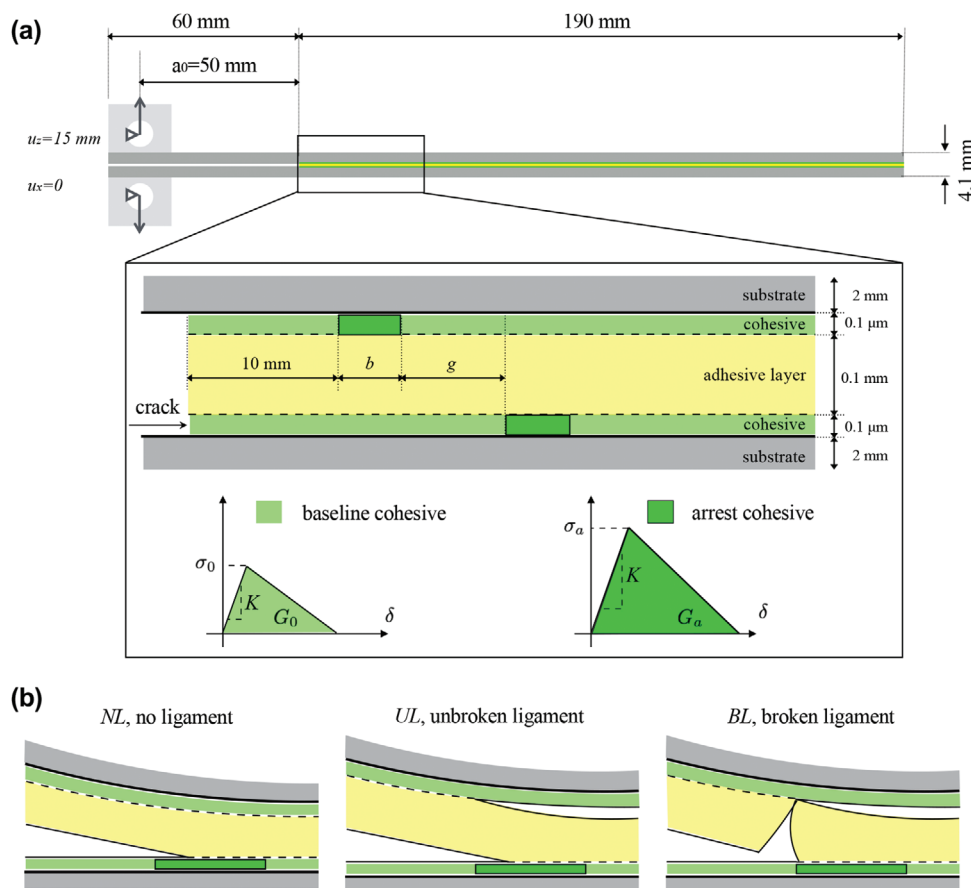
Figure 9. Techniques structuring the interface between the bondline and the substrate. a) Schematic of the 2D numerical model of surface alternative patterning strategy. The displacement control is applied to the bonding blocks. Parametric study included the patterning size b , gap distance g , baseline cohesive properties \sigma_0 , G_0 , and arrest cohesive properties \sigma_a , G_a . b) Schematic of three distinct failure modes depending on the interfacial properties: NL, UL, and BL. Reproduced with permission. [23] Copyright 2020, Elsevier B.V.
