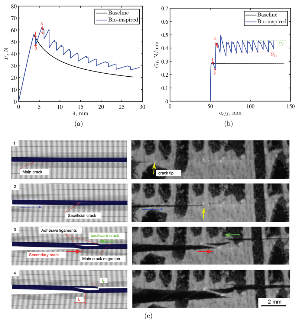
Figure 12. Subtractive techniques structuring the bondline. Damage evolution in bio-inspired adhesive joint: a) P - \delta curve, b) R-curve and c) damage modes at different loads marked in a. Reproduced with permission. [157] Copyright 2021, Elsevier B.V.
