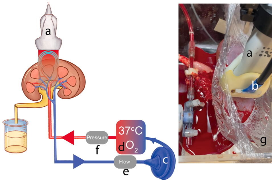
Fig. 1. The experimental PA NMP setup. (a) US transducer equipped with (b) laser fiber bundles. (c) Centrifugal pump head. (d) Oxygenator with a heat exchanger. (e) Flow sensor. (f) Pressure sensor. (g) Interface film filled with water.
