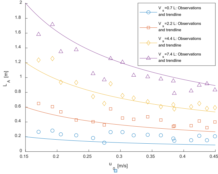
Figure 5. Observed carpet lengths, plotted for four driftwood volumes, decrease with increasing initial flow velocity. Fitted trendlines are of the shape L_A = \beta \cdot \frac{V_s}{u_0^\gamma} in Eq. (1) with \beta = 66.9 and \gamma = 0.74 .
