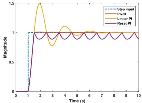
Figure 14: Step response of PI+CI, Linear PI and Reset PI
