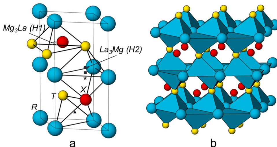
Fig. 2. a) Selected possible hydrogen sites in RTX hydride with TiNiSi-type related ZrBeSi-type structure. Interstitial sites: R_3T site ( \bullet ), R_3TX ( \blacksquare ), R_3X (*), R_2TX ( \blacktriangle ) and T_3R ( \circ ). The coordination polyhedra are outlined. Mg_3La (H1) and La_3Mg (H2) sites which are discussed in the Chapter 3.1 (Theoretical studies) are highlighted. (b) Structure of LaNiSnD_2 [6] illustrated as D ( La_3Ni ) tetrahedra sharing La–La edges and Ni corners. Isolated Sn atoms do not form bonds with hydrogen.
