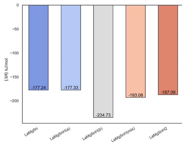
Fig. 5. Calculated formation energy ( \Delta H ) for LaMgSn, LaMgSnH [LaMgSnH (a) - H in a tetrahedral Mg 3 La site, LaMgSnH (b) - H in a tetrahedral La 3 Mg site, and LaMgSnH(mix) - H in both tetrahedral sites with an equal occupancy], and a hypothetical LaMgSnH 2 .
