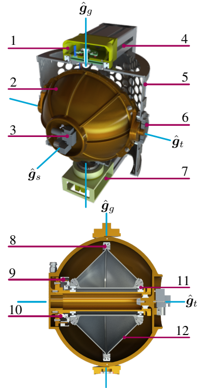
Fig. 2. The top figure shows a semi-cross-section of the whole device where (1) denotes the housing for the slip-ring and gimbal encoder, (2) the vacuum housing, (3) the vacuum-pump, (4) the device-frame, (5) the gimbal-frame, (6) the series coupling, and (7) the gimbal motor and gearbox. The bottom figure shows a cross-section of the sphere where (8) denotes the flywheel rim, (9) the electric motor, (10) The flywheel encoder, (11) the bearings, (12) the flywheel-sides.
