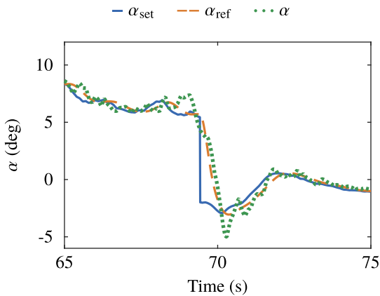
Fig. 13 Evolution of the angle of attack with set point \alpha_{\text{set}} , reference filter state \alpha_{\text{ref}} , and achieved angle of attack \alpha .
