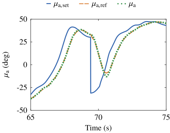
Fig. 12 Evolution of the aerodynamic bank angle. Set point \mu_{a,\text{set}} , reference \mu_{a,\text{ref}} , and achieved bank angle \mu_a .
