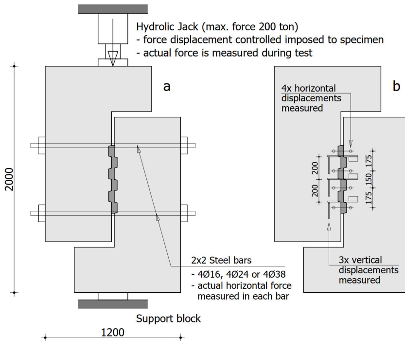
Figure 4.13: Overview of the test setup (a) and measurements (b), measures in mm
