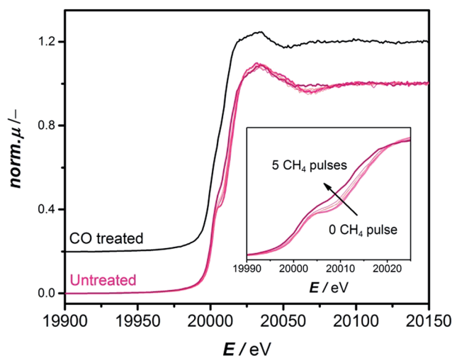
Fig. 3 Comparison of operando XANES spectra recorded at Mo K-edge for a 2MoHZ-13 catalyst during consecutive pulsing of \text{CH}_4 at 700^\circ\text{C} (pink curves) and a 2MoHZ-13 catalyst carburized at 780^\circ\text{C} with a 30 \text{ ml min}^{-1} flow of 2.5% CO in He (black curve).
