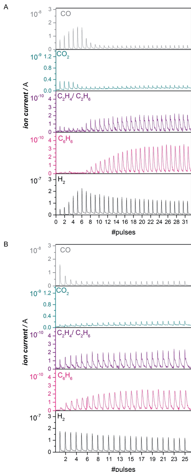
Fig. 2 Evolution of CO, \text{C}_2\text{H}_4/\text{C}_2\text{H}_6 , \text{CO}_2 , \text{C}_6\text{H}_6 and \text{H}_2 with a consecutive pulsing of 223 \mu\text{mol CH}_4 at 700^\circ\text{C} to 300 mg of an untreated 2MoHZ-13 (Panel A) and the same catalyst pre-carburized with a 30 \text{ ml min}^{-1} flow of 2.5% CO in He at 780^\circ\text{C} for 1 h (Panel B).
