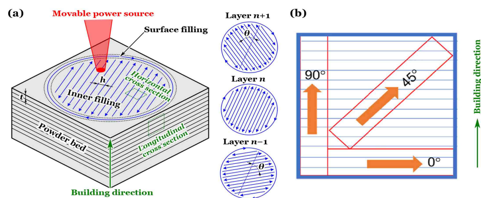
Figure 1. (a) Schematic drawing for powder bed fusion (PBF) with a scan strategy of meandering paths [15]. (b) The 3D printed specimens [16] with orientations of 0°, 45°, and 90°.
