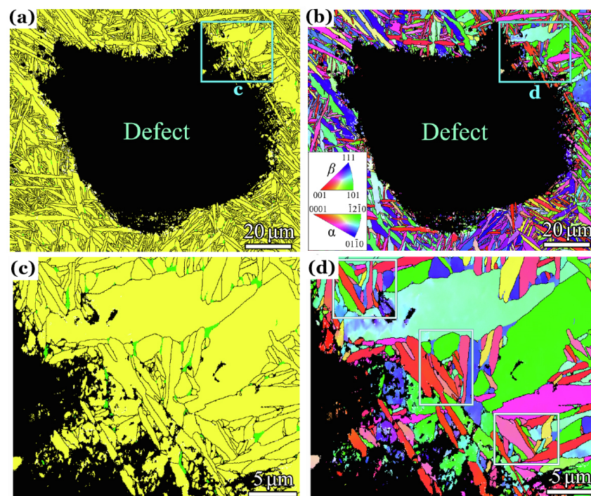
Figure 6. Electron backscatter diffraction (EBSD) for an additively manufactured titanium alloy with Group 12 of processing parameters via laser powder bed fusion and experienced through annealing [57]: (a) Phase map, yellow for \alpha and cyan for \beta ; (b) Inverse pole figure (IPF) showing crystallographic orientations of \alpha and \beta grains. (c,d) enlarging boxes c and d in (a,b).
