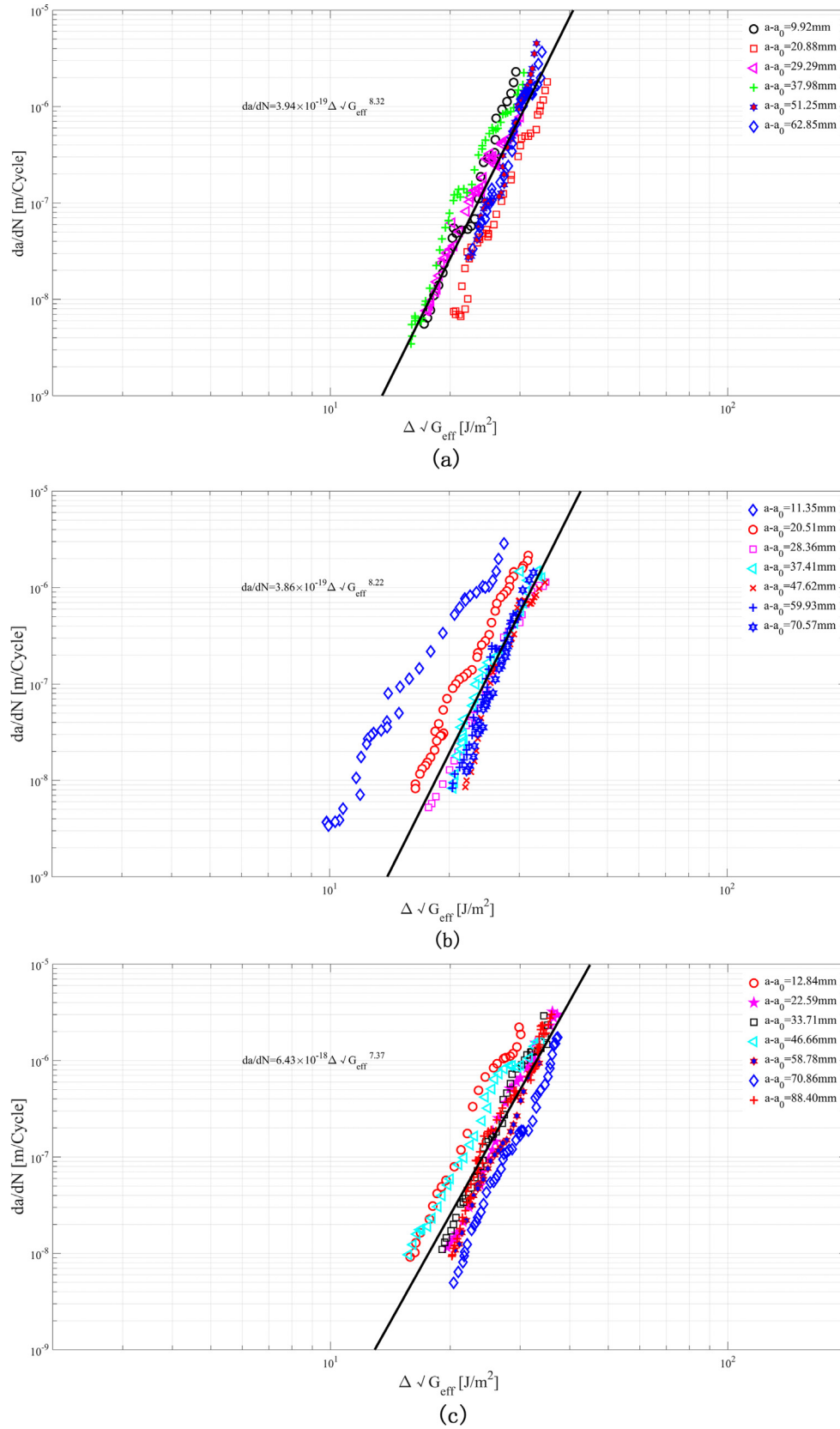
Fig. 11. Fatigue delamination interpreted via the modified Paris relation (a) Sp-32-01; (b) Sp-32-02; (c) Sp_48. (For interpretation of the references to colour in this figure legend, the reader is referred to the web version of this article.)
